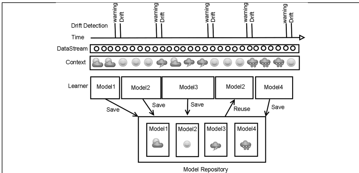
Fig. 1. Context-aware data stream learning system. (Colours are visible in the online version of the article; http://dx.doi.org/10.3233/IDA-2012-0552 )
