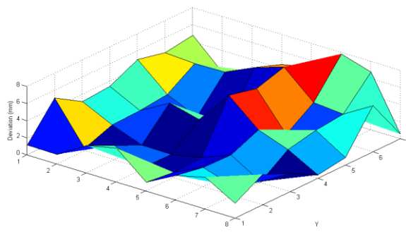
Fig. 4. Accumulated distance error. The error increases with regard to the distance from the first row of the measurement plate.
