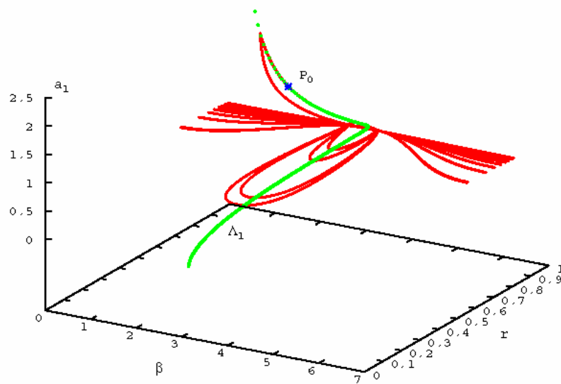
Figure 5. Projection on space \beta - r - a_1 of the 4-periodic orbit and the curve \Lambda_l for \Gamma = 0.001 , \gamma_2/\gamma_3 = 0.999580176 , \gamma_2 = 1 and \nu = 1.5 .
