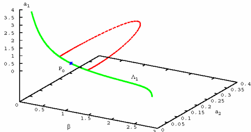
Figure 4. Projection on space \beta - a_2 - a_1 of the periodic orbit and the curve \Lambda_l for \Gamma = 0.001 , \gamma_2/\gamma_3 = 0.99957616 , \gamma_2 = 1 and \nu = 1.5 .
