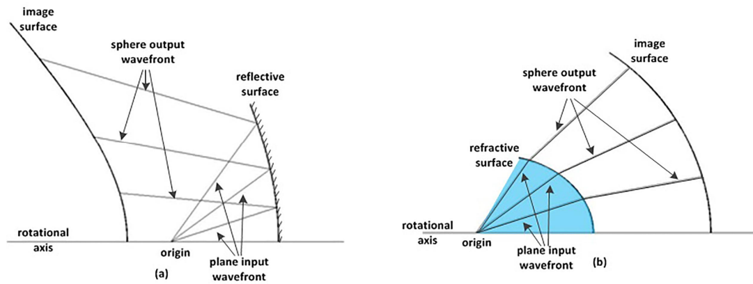
Figure 2. The reflective anastigmatic rotational design (a) and the refractive anastigmatic rotational design (b). The image surface profile is calculated after the design of the optical surface
