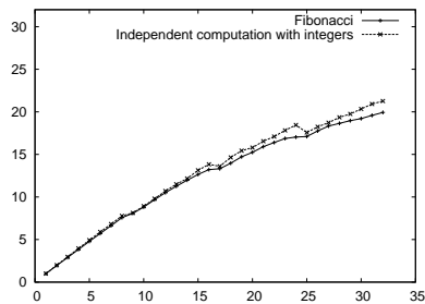
Fig. 10. Fibonacci with gran. control vs. maximum speedup in real machine.
