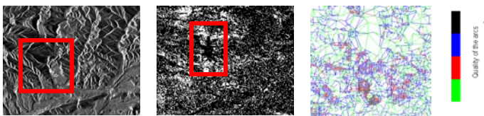
Figure 6. Amplitud image, selected pixels using the coherence criterion and Delaunay triangulations of study area (red square). Line colour indicates for the
