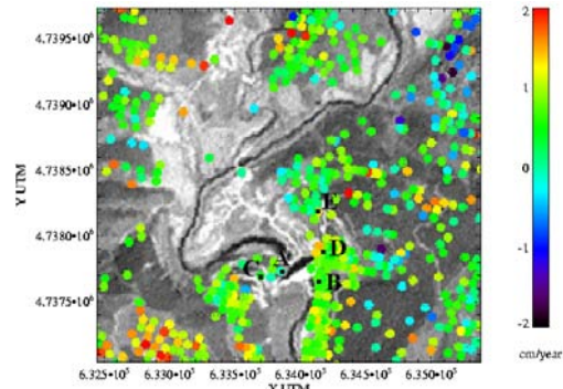
Figure 7. Deformation map. Darker colour means positive and softer colour means negative LOS velocity of displacements.
