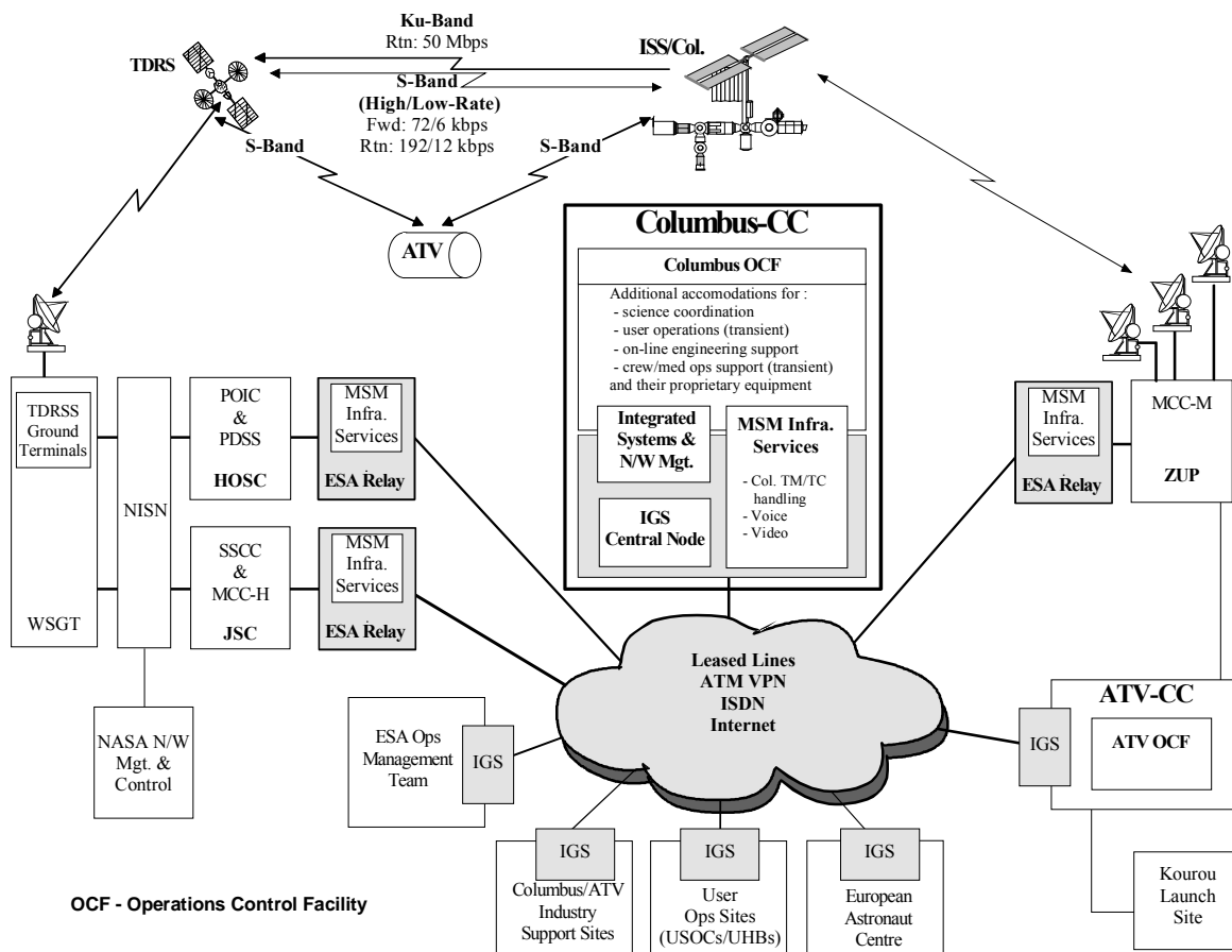
Figure 2.2. Columbus Ground Segment
