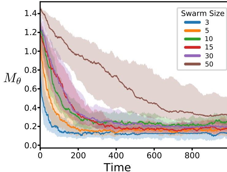
Figure 4.28: Scalability assessment in the orientation consensus primitive. Evolution of the misalignment metric ( M_\theta ) for different swarm sizes. The darker curves represent the median value of M_\theta , and the boundaries of the shadow areas indicate the first and third quartiles. Fifty independent simulations are used for each swarm size.
