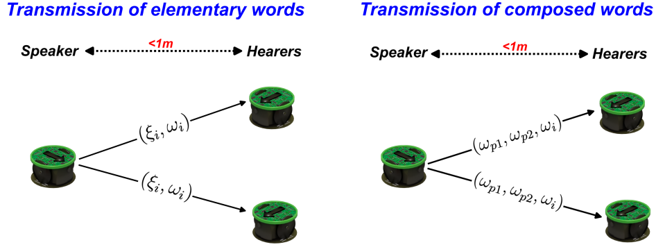
Figure 6.12: Overview of the customized naming game used in the experiment. Unidirectional interactions among a single speaker and multiple hearers during language games. It shows two possible types of transmissions with elementary and composed words.
