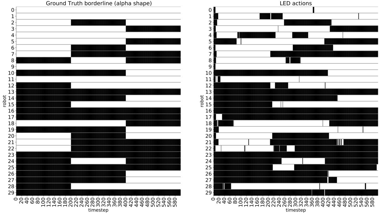
Figure 4.21: Robustness assessment in the frontier identification task. The topology of the robot swarm is drastically changed every 200 control cycles. (A) Ground truth LED actions according to the alpha shape algorithm. (B) Evolution of the actual LED actions of the robots. Black bars indicate that the LED is turned on and blank spaces represent LEDs turned off.
