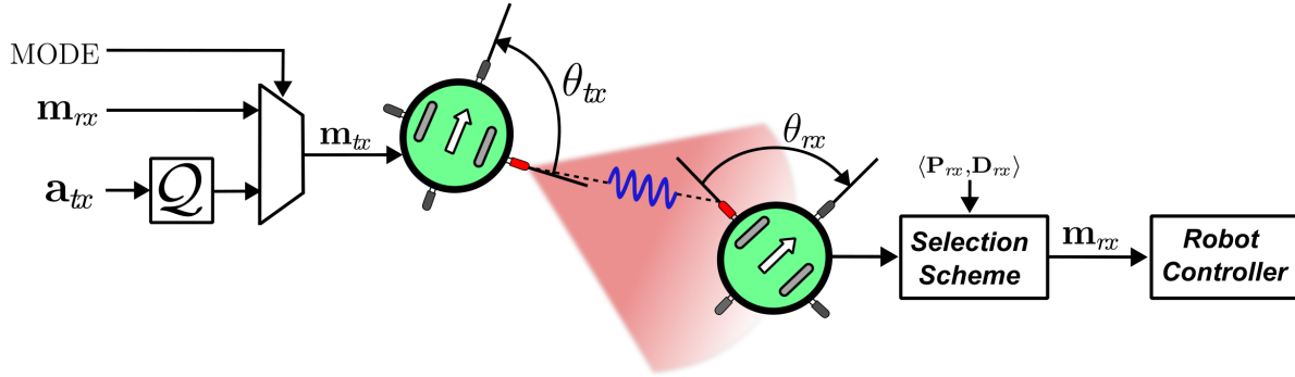
Figure 4.4: Overall diagram of the communication system
