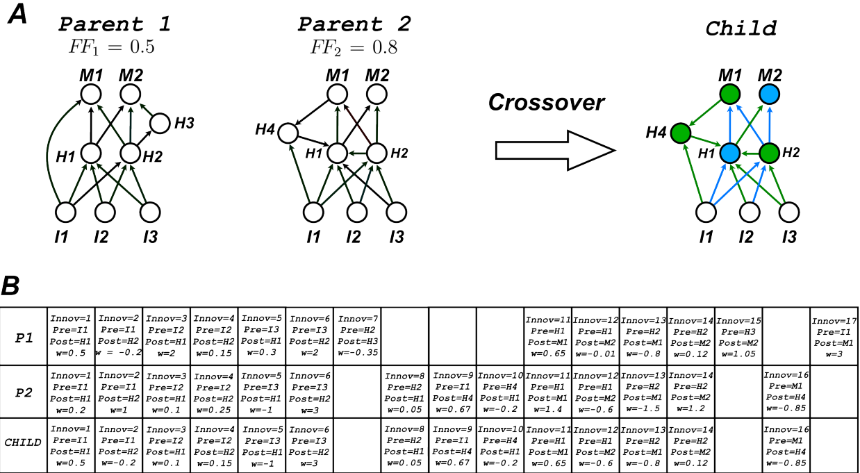
Figure A.5: Example of the NEAT crossover operator. (A) ANN architectures of the parents genotypes and the child resulting from the crossover. For each parent the hypothetical fitness score FF_i is displayed, showing that the fittest parent is Parent 2. The color of the neurons and synapses of the child ANN indicate the parent from whom the corresponding gene was inherited (blue for Parent 1 and green for Parent 2). According to [83], topological genes (connections and nodes) are inherited from the parent with highest fitness score (Parent 2 in this example). (B) List of connection genes of both parents and the resulting child.
