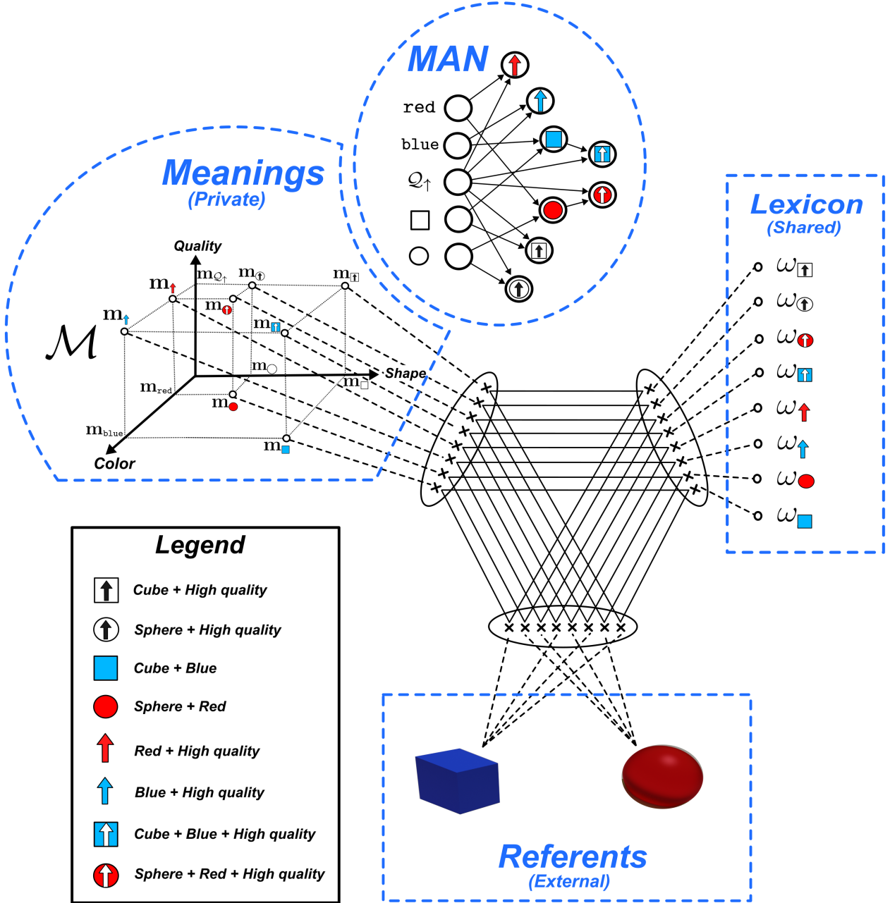
Figure 6.10: General diagram of the complete semiosis process of composed semiotic symbols. It shows the different sets that constitute the triad of a composed semiotic symbols (referents, meanings, and forms), in blue. The diagram shows an example with two different geometric objects: high quality blue cube, and high quality red sphere. Furthermore, the MAN is shown alongside the meanings, indicating how compositionality is defined.
