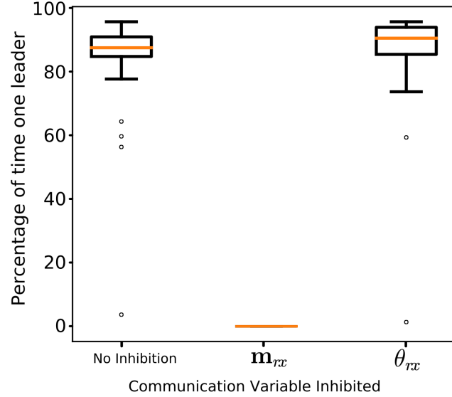
Figure 4.14: Box plot of the percentage of the total simulation time with a single leader in simulations when different variables are inhibited. Each box plot is constructed using data from 50 independent simulations.
