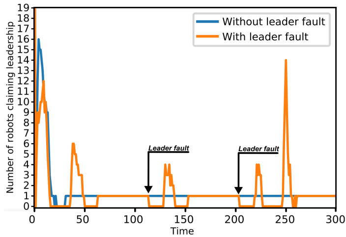
Figure 4.12: Temporal evolution of the number of robots claiming leadership for a trajectory in normal conditions and with leader failure.
