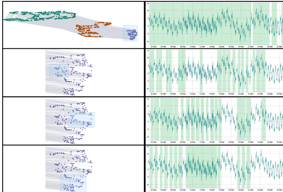
Figure A.11: Cluster I: Zoom in the first cluster of the execution of MOMENT-base for S1. No clear segmentation detected.
