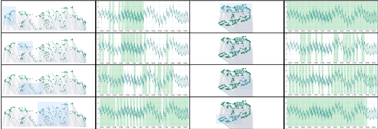
Figure A.13: Cluster III: Zoom in the third cluster of the execution of MOMENT-base for S1. Detects df_2 .
