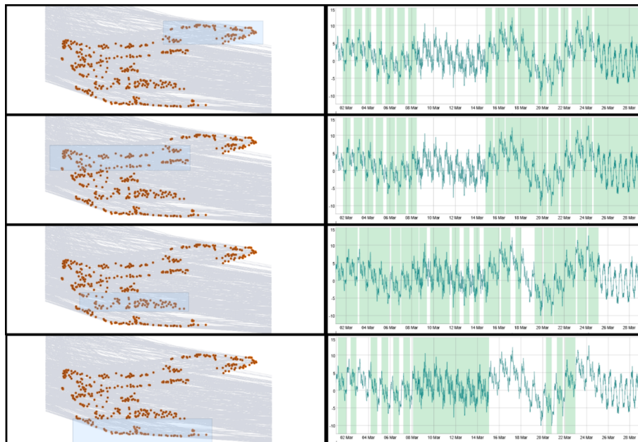
Figure A.12: Cluster II: Zoom in the second cluster of the execution of MOMENT-base for S1. Close to detect df_2
