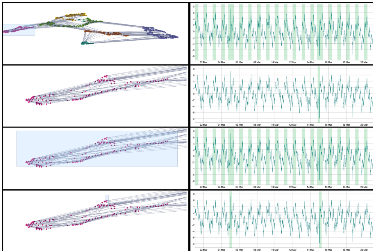
Figure A.16: Cluster I: Analysis of the first cluster in the embeddings projections of the zero-shot version of MOMENT-large applied to S2.
