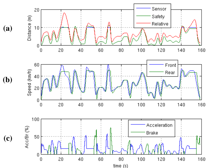
Figure 2. Result of a simulation with the controller obtained by the Genetic Algorithm. (a) Distance between vehicles, distance measured with the ultrasonic sensor (between 1 and 10 m), and braking distance. (b) Speed of both vehicles. (c) Actions on accelerator and brake.
