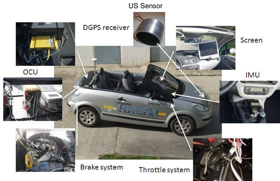
Figure 8. Experimental prototype.
