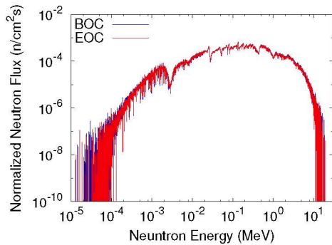
FIG. 1. ESRF neutron spectra at BOC and EOC.
