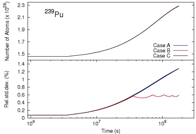
FIG. 2. Number of atoms of 239 Pu throughout the burn-up and its uncertainty for each of the cases studied using EAF-2010+SCALE uncertainties.
