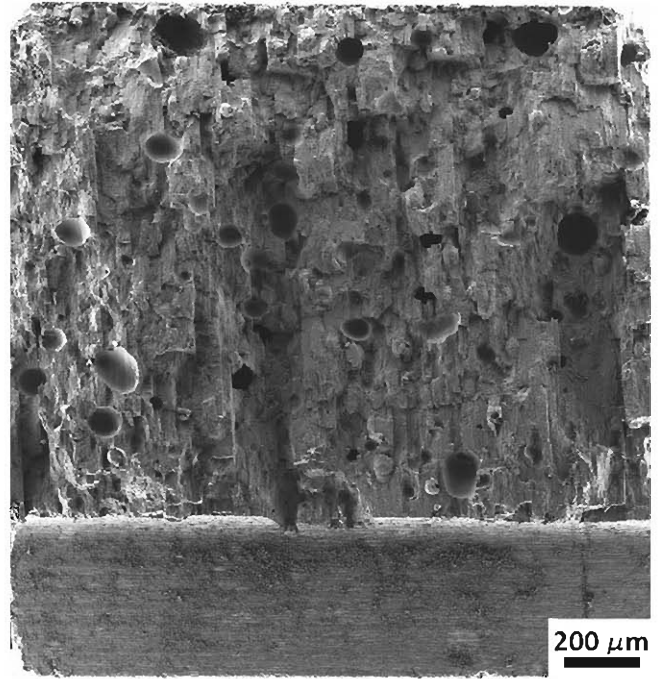
Figure 17. Fracture surface of GdBCO/Ag single grain after the three-point bending test for the measurement of fracture toughness at 77 K. The loading direction was parallel to the ab -plane. Brittle fracture and abrupt fracture surface is observed.
