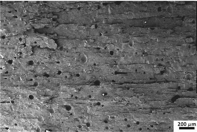
Figure 20. Fracture surface of the GdBCO/Ag single grain after the splitting test at 77 K. The propagation of the cracks is parallel to the ab -plane and the density of cracking produced narrow superconducting areas within the sample.
