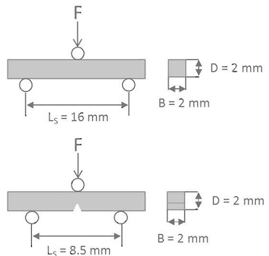
Figure 2. Schematic illustration of the three-point bending tests for evaluation of the flexural strength and fracture toughness.
