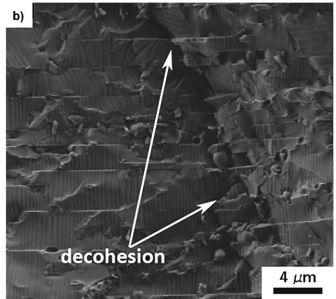
Figure 14. Fracture surface of the YBCO single grain after the three-point bending test for the measurement of fracture toughness at 77 K. The loading direction was parallel to the c -axis. (a) Propagation of the crack perpendicular to the ab -plane and (b) Decohesion of the grain.
