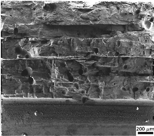
Figure 13. Fracture surface of the YBCO single grain after the three-point bending test for the measurement of fracture toughness at 77 K. The loading direction was parallel to the c -axis.
