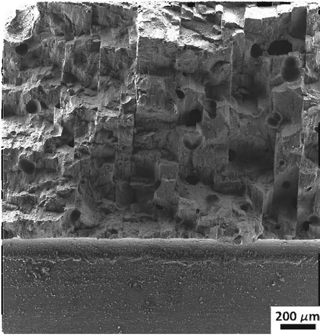
Figure 15. Fracture surface of the YBCO single grain after the three-point bending test for the measurement of fracture toughness at 77 K. The loading direction was parallel to the ab -plane. Brittle fracture and a curved fracture surface are observed.
