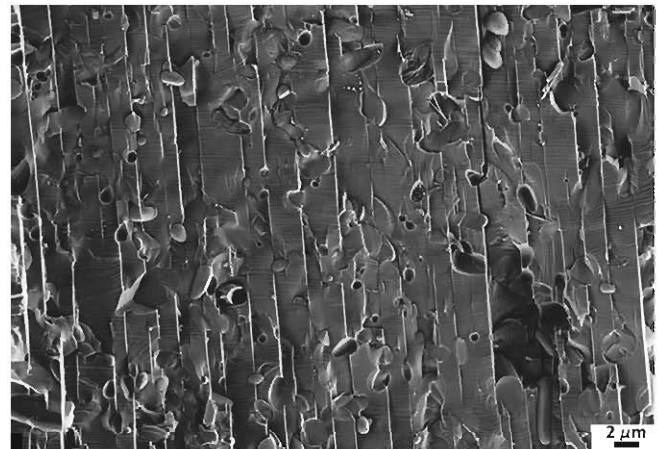
Figure 11. Fracture surface of GdBCO/Ag single grain after the three-point bending test for the measurement of flexural strength at 77 K. The loading direction was parallel to the ab -plane. Cracks propagate through the pre-existing microcracks and around the Gd-211 secondary phase inclusions.
