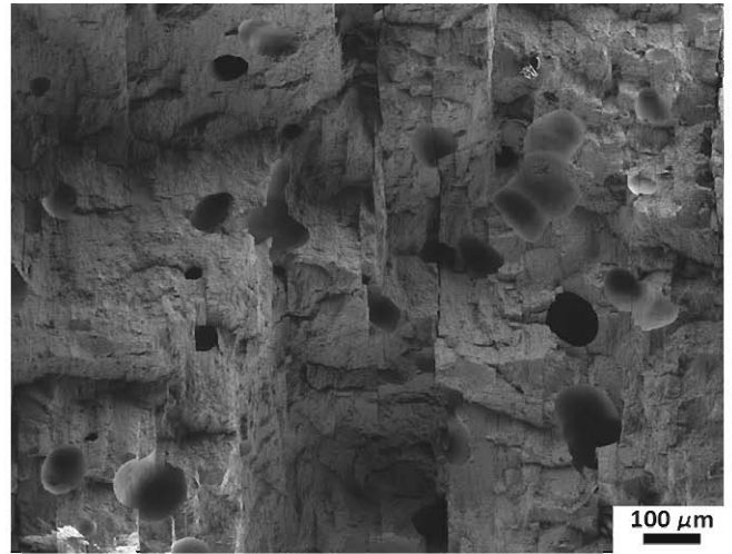
Figure 8. Fracture surface of YBCO single grain after the three-point bending test for the measurement of flexural strength at 77 K. The loading direction was parallel to the ab -plane. The propagation of the crack parallel to the ab -plane and the density of voids are indicated.
