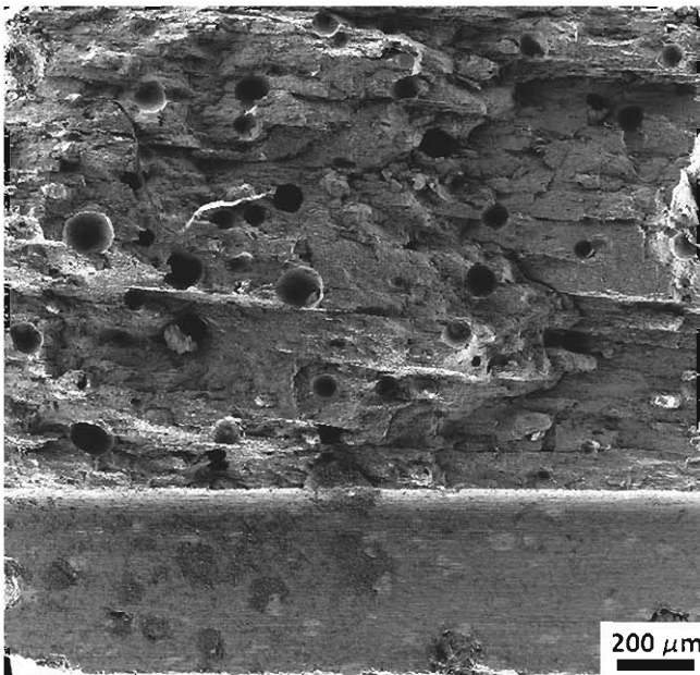
Figure 16. Fracture surface of GdBCO/Ag single grain after the three-point bending test for the measurement of fracture toughness at 77 K. The loading direction was parallel to the c -axis. A change in the direction of the propagation of the main crack is observed.
