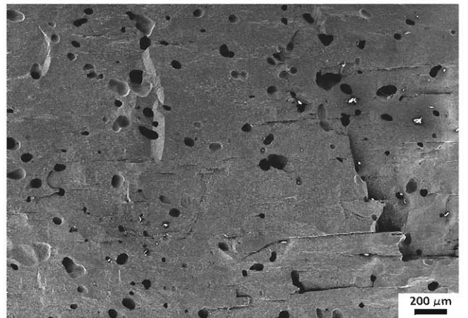
Figure 18. Fracture surface of the YBCO single grain after the splitting test at 77 K. The propagation of cracks parallel to the ab -plane and the density of voids can be seen.
