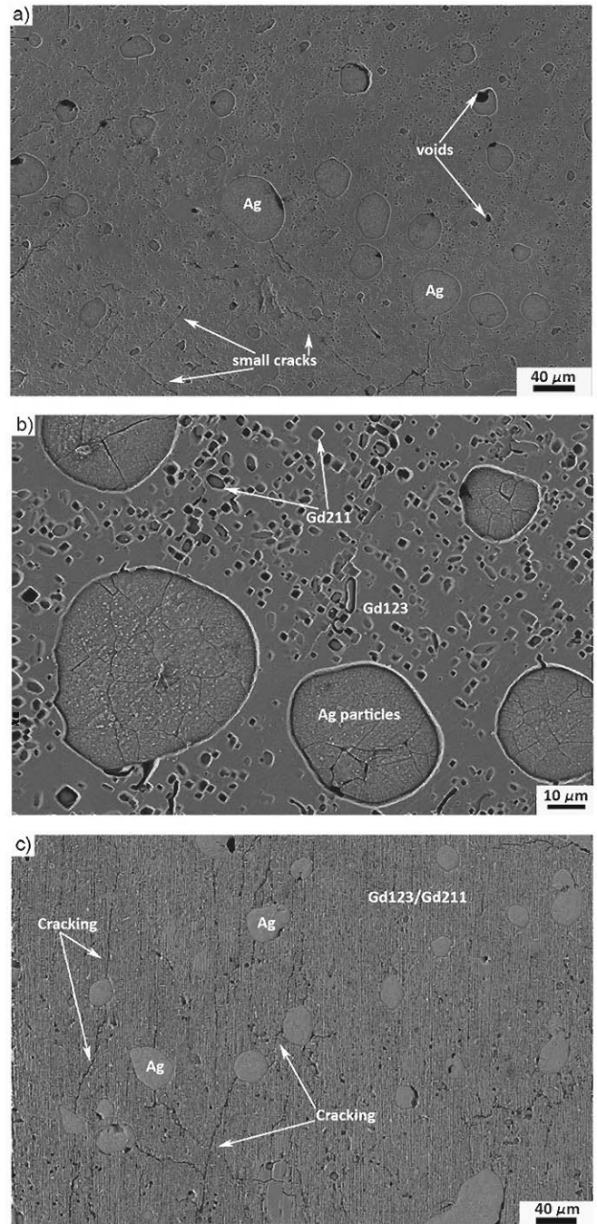
Figure 5. (a) Microstructure of the longitudinal section of the GdBCO/Ag 15 wt% single grain. Small cracks, voids and the size of Ag particles are indicated. (b) Microstructure of the longitudinal section of the GdBCO/Ag 15 wt% single grain. The secondary phase of Gd-211 and the size of Ag particles are indicated. (c) Microstructure of the transversal section of the GdBCO/Ag 15 wt% single grain. Cracking parallel to the ab -plane and around the Ag particles can be seen.
