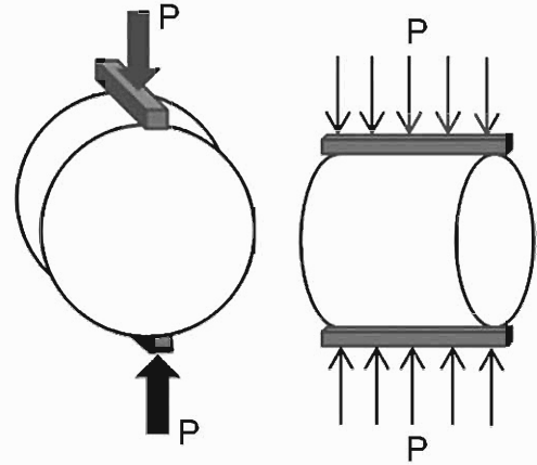
Figure 3. Schematic illustration of the Brazilian test for evaluation of tensile strength.
