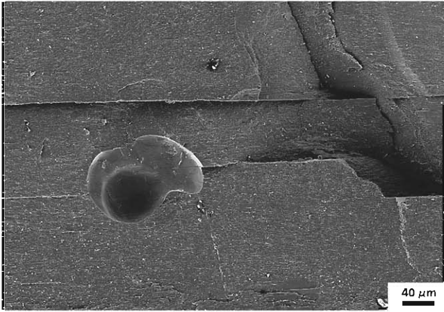
Figure 19. Fracture surface of the YBCO single grain after the splitting test at 77 K. Cracks propagate mainly parallel to the ab -plane, although perpendicular cracks that led to the fracture can be observed.
