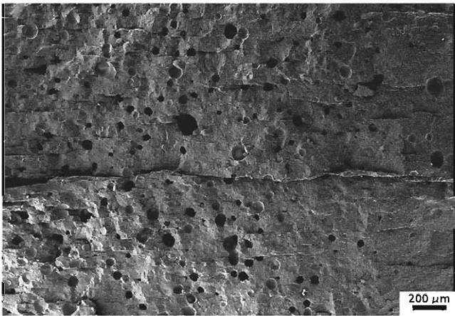
Figure 21. Fracture surface of the GdBCO/Ag single grain after the splitting test at 77 K. The propagation of the cracks is parallel to the ab -plane and the fracture is more abrupt than in the case of YBCO.
