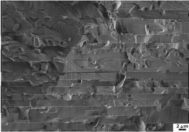
Figure 9. Fracture surface of GdBCO/Ag single grain after the three-point bending test for the measurement of the flexural strength at 77 K. The loading direction was parallel to the c -axis. A smooth fracture surface and the propagation of cracks perpendicular to the ab -plane are observed.
