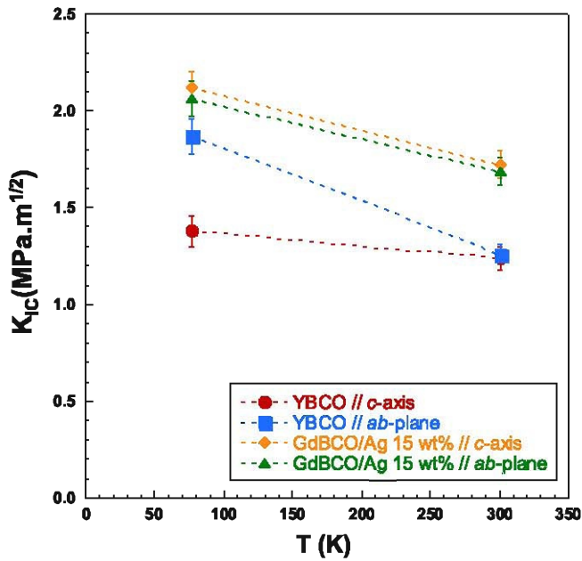
Figure 12. Variation of the fracture toughness as a function of temperature and loading direction. Each point represents the value of the mean of ten tests, and the bars indicate mean quadratic error.
