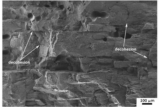
Figure 7. Fracture surface of the YBCO single grain after the three-point bending test for the measurement of flexural strength at 77 K. The loading direction was parallel to the c -axis. Decohesion and fracture of the domain are shown in the figure.
