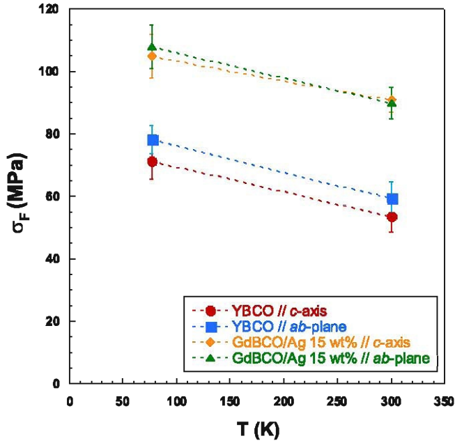
Figure 6. Variation of flexural strength as a function of temperature and test direction. Each point represents the mean value of the results of ten tests. The bars indicate the quadratic mean error.
