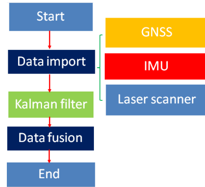
Fig. 11: Data processing
