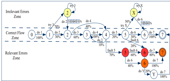
Figure 1: Example of an extended automata
