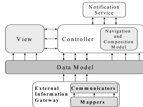
Figure 2. ODESeW extended-MVC design pattern.
