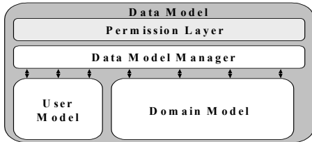
Figure 1. The ODESeW Data Model and its components.
