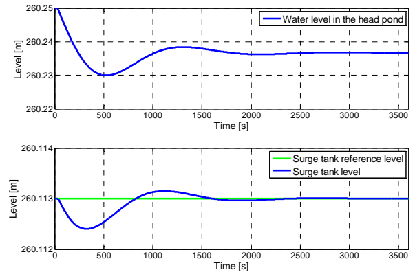
Figure 3: Head pond and surge tank water levels.
