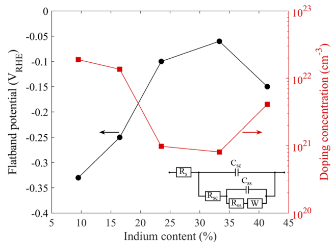
FIG. 6. Flatband potential (left y-axis) and doping concentration (right y-axis) of \text{In}_x\text{Ga}_{1-x}\text{N} water-splitting photoelectrodes determined by the Mott–Schottky analysis (Fig. S10 in the supplementary material). The equivalent circuit for the electrochemical impedance spectrum fit is also indicated.
