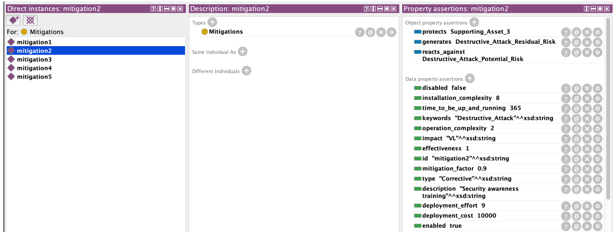
Figura 9.24: Mitigación 2 - Destructive Attack
