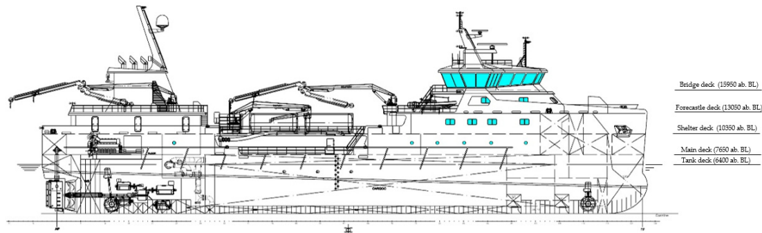
Figure 1. General arrangement of the 3000 m 3 wellboat.
