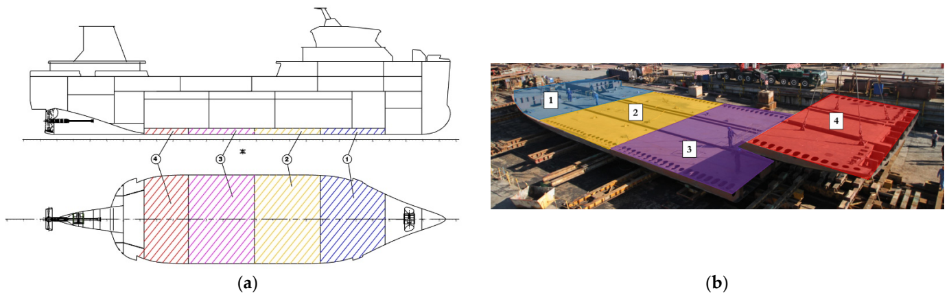
Figure 4. (a) General view of double-bottom tanks and (b) construction process of double-bottom tanks.
