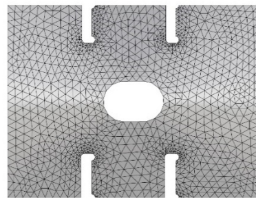
Figure 13. Mesh pattern.
