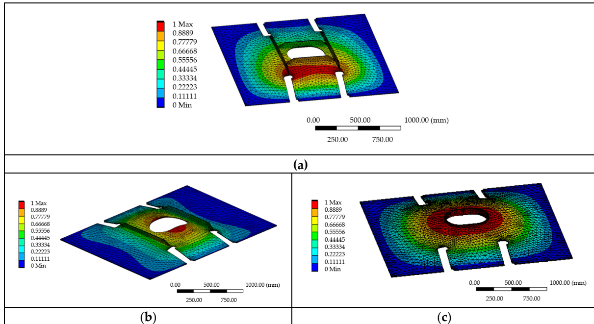
Figure 20. Buckling modes (mm): (a) Stiffening technique b80 \times 12 (mm) under transverse compression, (b) stiffening technique a70 \times 10 (mm) under longitudinal compression and (c) stiffening technique d80 \times 14 (mm) under biaxial compression.
