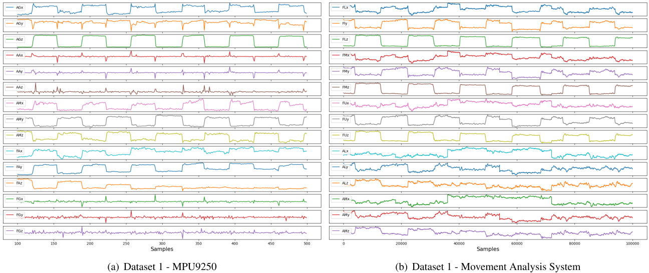
FIGURE 8. Signals from dataset 1 MPU9250 and visual markers.
