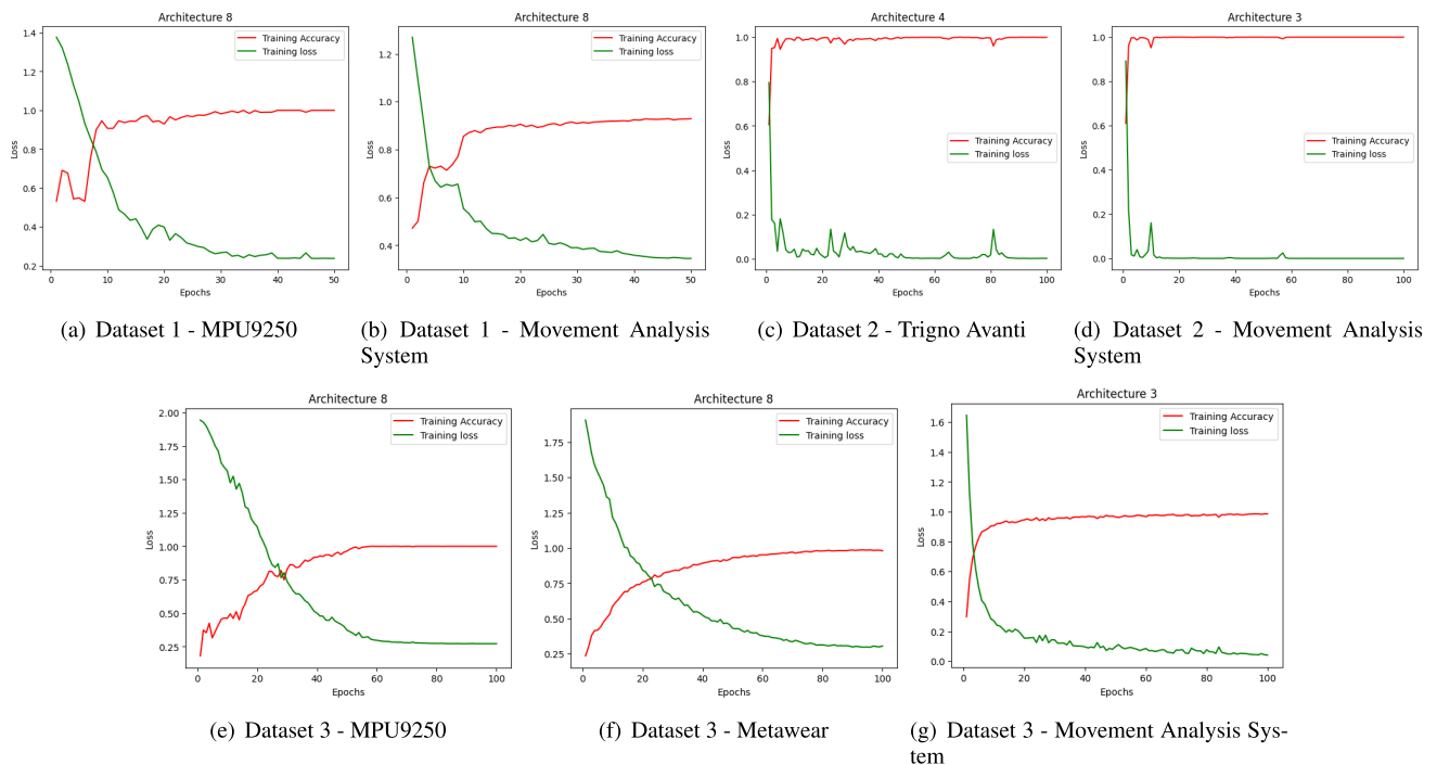
FIGURE 15. Plot of best architectures for every dataset using best features.
