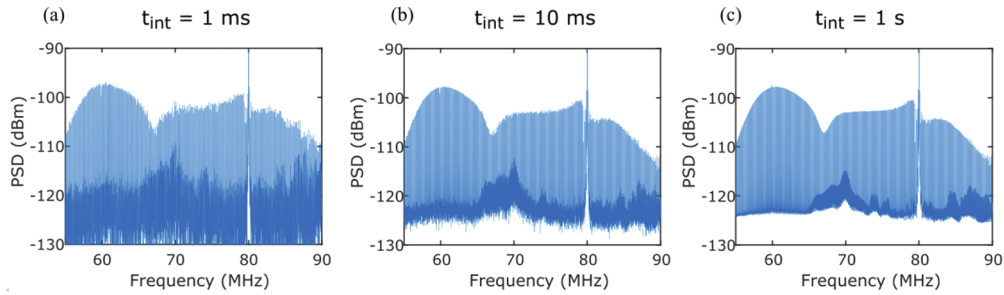
Fig. 4. Down-converted RF combs measured with the oscilloscope when the light goes through the \text{H}^{13}\text{CN} cell for three different integration times: 1 ms (a), 10 ms (b) and 1 s (c). The vertical scale is reduced to magnify the view of the spectra (the injection peak had an amplitude of \sim 70 dBm).
