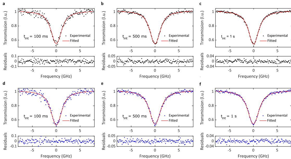
FIGURE 7. Transmission profiles of the \text{H}^{13}\text{C}^{14}\text{N}(10) line. The black dots plot the profile obtained experimentally and the solid red line corresponds to the Voigt profile fitted to these data. The residuals from the fitting are shown in the bottom part of each figure. The results acquired using the oscilloscope to digitize the data are shown in the top row for integration times ( t_{\text{int}} ) of: a, 100 ms; b, 500 ms and c, 1 s. The transmittances obtained for these same integration times when the acquisition is performed with the SDR platform are shown in the bottom row: d, e and f.
