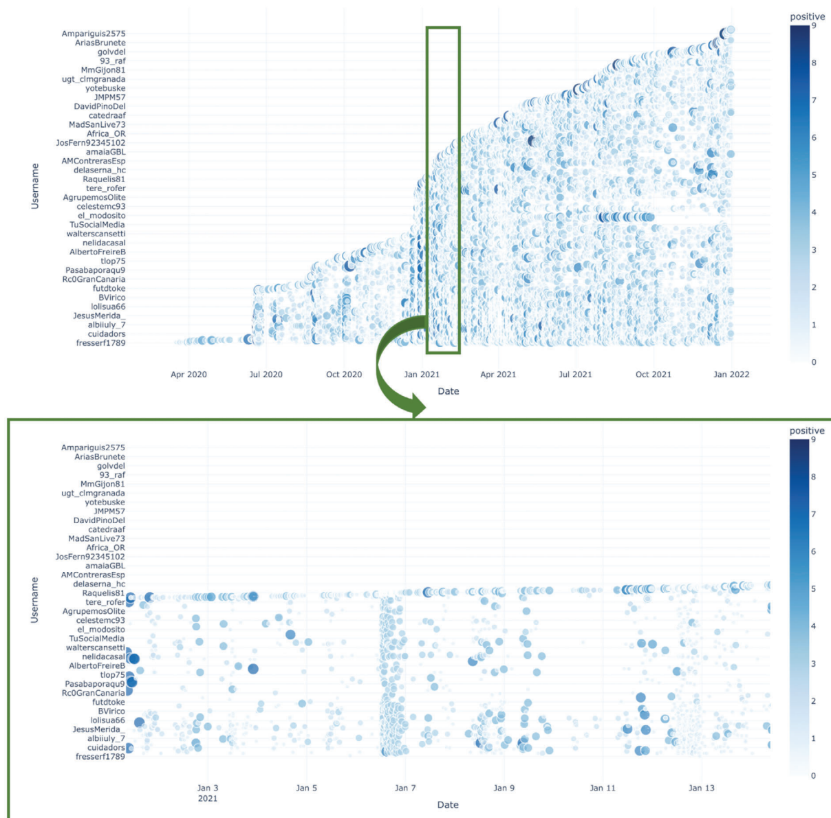
Fig. 8. Tweets by date.
