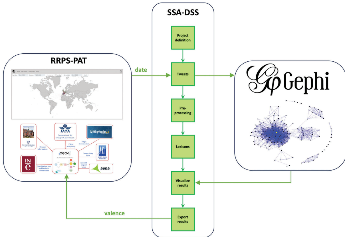
Fig. 1. Integration of SSA-DSS with the RRPS-PAT module and Gephi.
