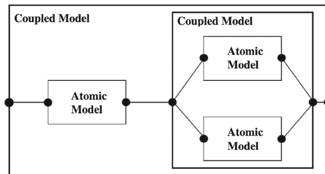
FIGURE 1 Hierarchical DEVS model with atomic and coupled components and associated couplings
