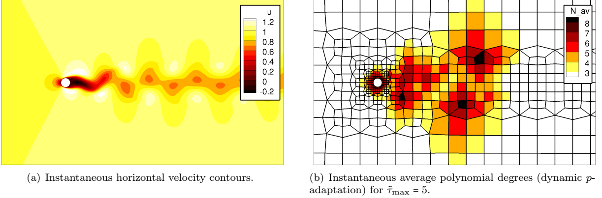
Figure 8: Vortex shedding behind a cylinder at Re_\infty = 100 .
