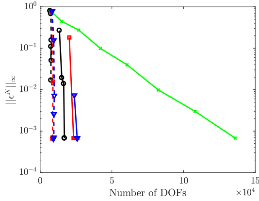
(a) Maximum error vs. number of DOFs.
