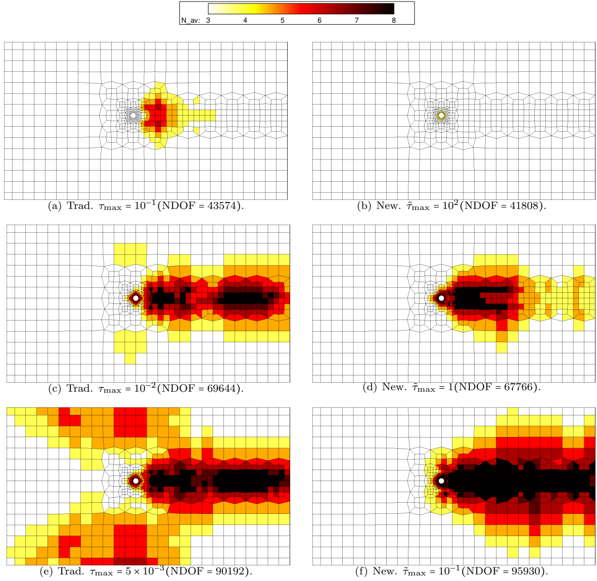
Figure 9: Comparison of the two possible formulations of the truncation error: traditional (left) and new (right). Average polynomial degree distribution for static p -adaptation for different error thresholds.
