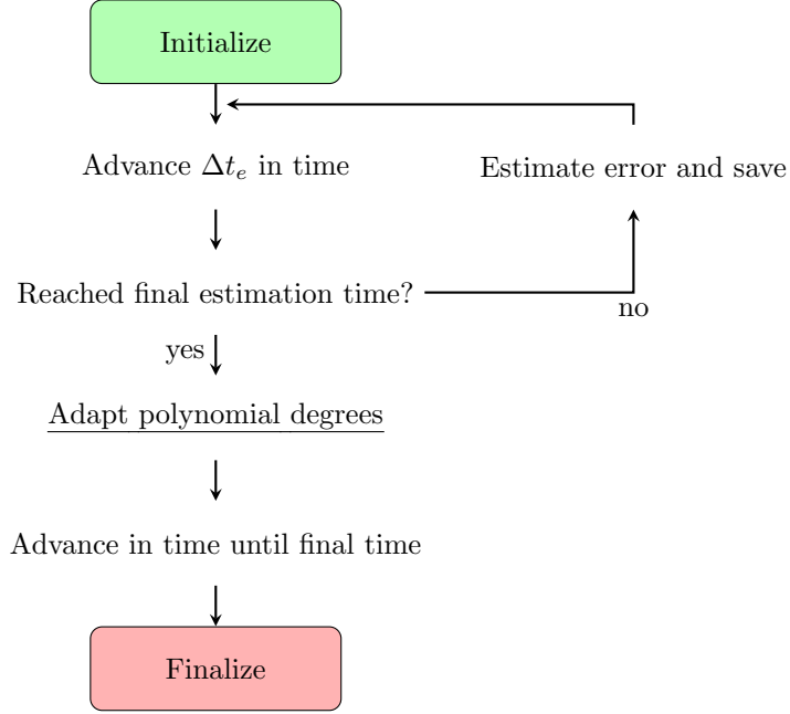
Figure 2: Flowchart of the static p -adaptation.
