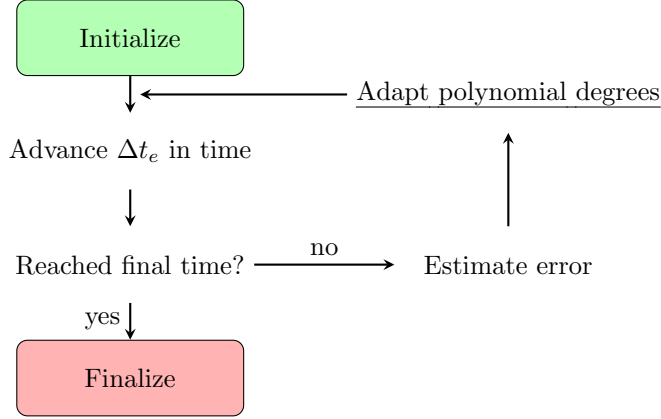
Figure 1: Flowchart of the dynamic p -adaptation.
