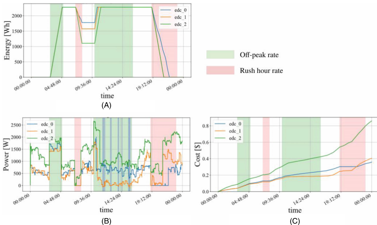
FIGURE 15 Battery energy storage, grid power consumption and energy cost. (A) Energy stored per EDC, (B) power consumption drawn from the power grid per EDC, (C) energy cost profile per EDC.
