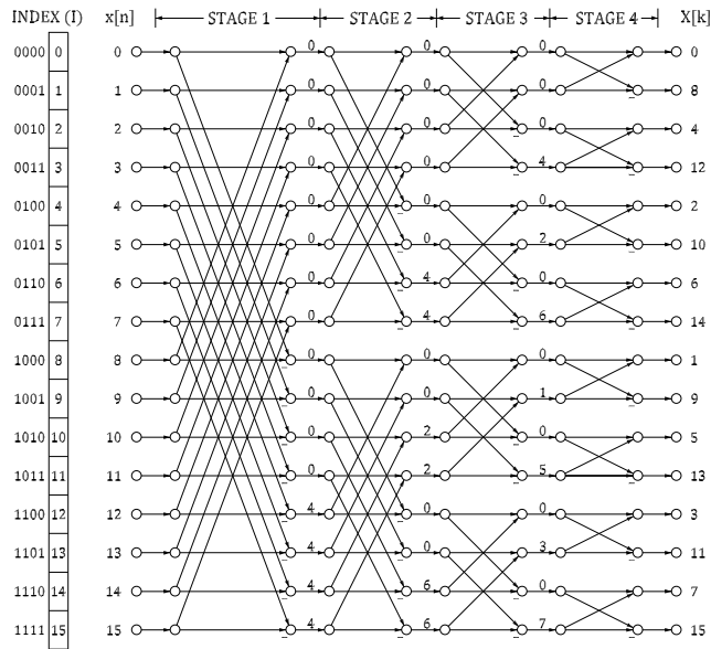
Fig. 2: Flow graph of a 16-point radix-2 DIT FFT.
