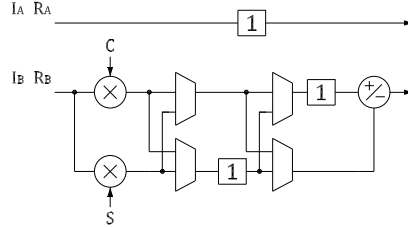
Fig. 24: Alternative rotator in an radix-2 SDC FFT architecture that divides the data in real and imaginary parts.
