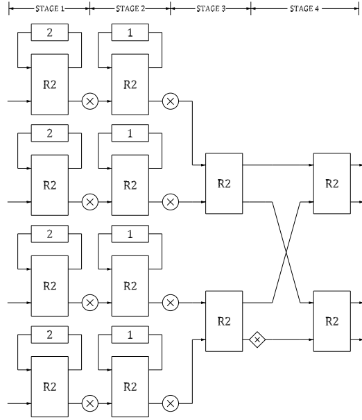
Fig. 32: 16-point 4-parallel radix-2 MDF FFT architecture.
