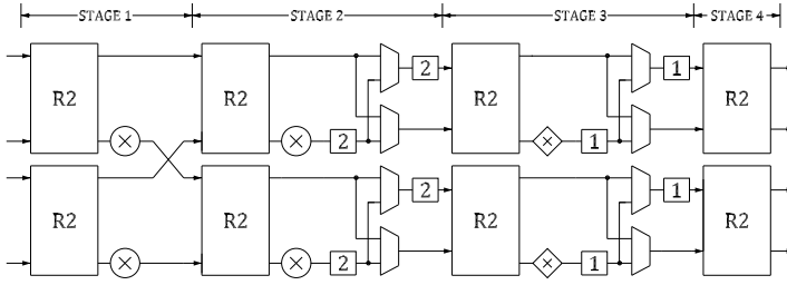
Fig. 36: 16-point 4-parallel radix-2 MDC FFT architecture.
