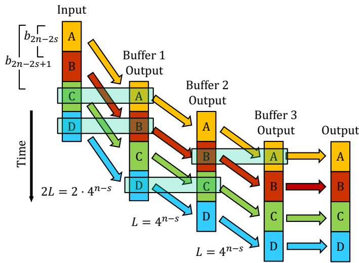
Fig. 16: Timing of a deep feedback radix-2 SDF FFT architecture.
