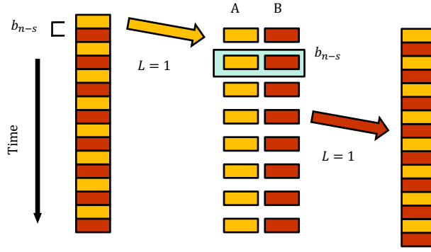
Fig. 28: Timing of a radix-2 SC FFT architecture.
