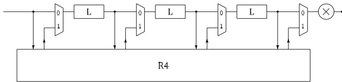
Fig. 11: Stage of a radix-4 SDF FFT architecture.
