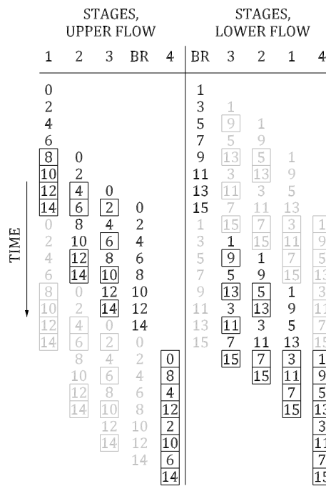
Fig. 35: Timing of a 16-point 2-parallel radix-2 M^2DF FFT architecture.
