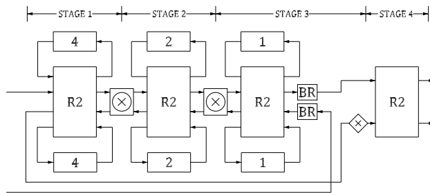
Fig. 34: 16-point 2-parallel radix-2 M^2DF FFT architecture. The boxes labeled with BR are circuits to calculate the bit reversal [31].
