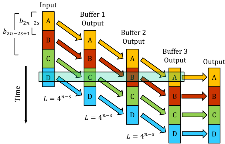
Fig. 12: Timing of a radix-4 SDF FFT architecture.
