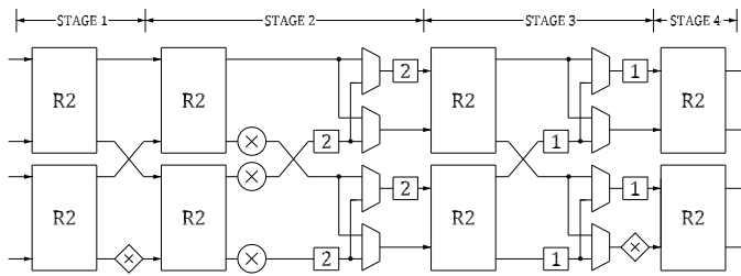
Fig. 40: 16-point 4-parallel radix- 2^2 MDC FFT architecture.
