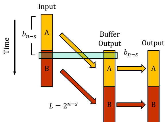
Fig. 9: Timing of a radix-2 SDF FFT architecture.
