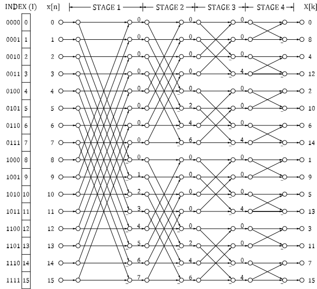
Fig. 1: Flow graph of a 16-point radix-2 DIF FFT.
