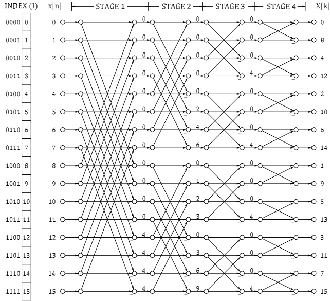
Fig. 5: Flow graph of a 16-point radix- 2^2 FFT.
