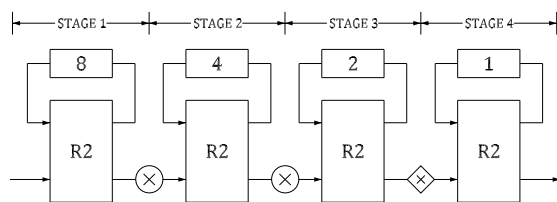
Fig. 7: 16-point radix-2 SDF FFT architecture.
