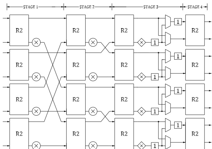
Fig. 38: 16-point 8-parallel radix-2 MDC FFT architecture.
