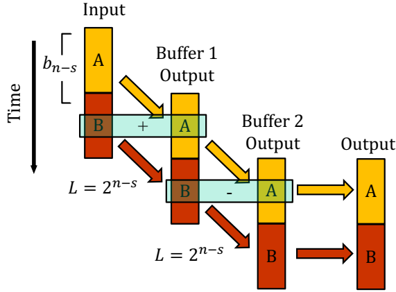
Fig. 26: Timing of a radix-2 SFF FFT architecture.
