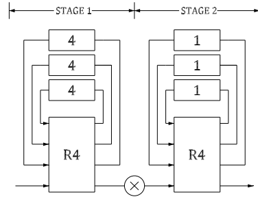
Fig. 10: 16-point radix-4 SDF FFT architecture.
