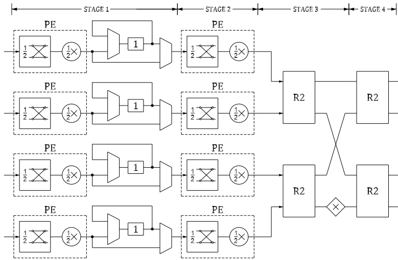
Fig. 44: 16-point 4-parallel radix-2 MSC FFT architecture.
