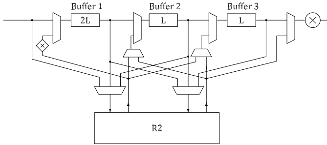
Fig. 15: Stage of a deep feedback radix-2 SDF FFT architecture.
