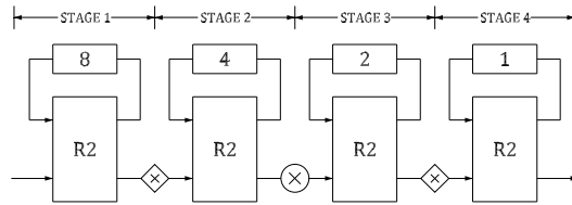
Fig. 13: 16-point radix- 2^2 SDF FFT architecture.
