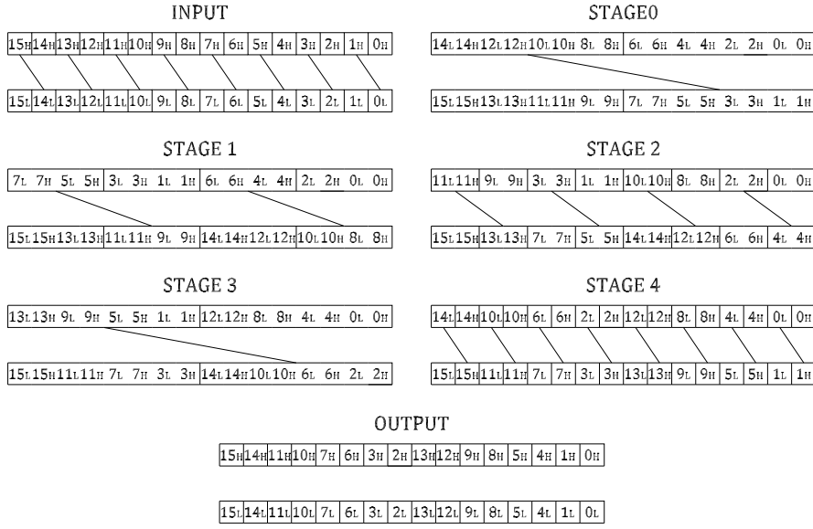
Fig. 21: Timing of a 16-point 2-parallel radix-2 SDC FFT architecture that divides the data in high and low parts.
