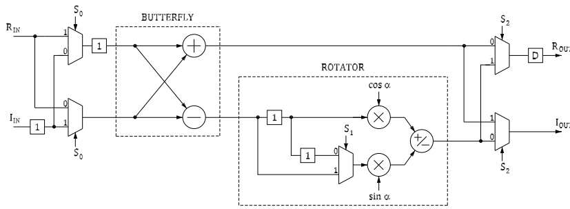
Fig. 29: Stage of an SC FFT architecture.
