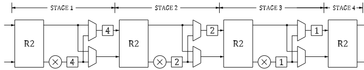
Fig. 17: 16-point 2-parallel radix-2 MDC FFT architecture.
