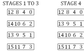
Fig. 33: Timing of a 16-point 4-parallel radix-2 MDF FFT architecture.
