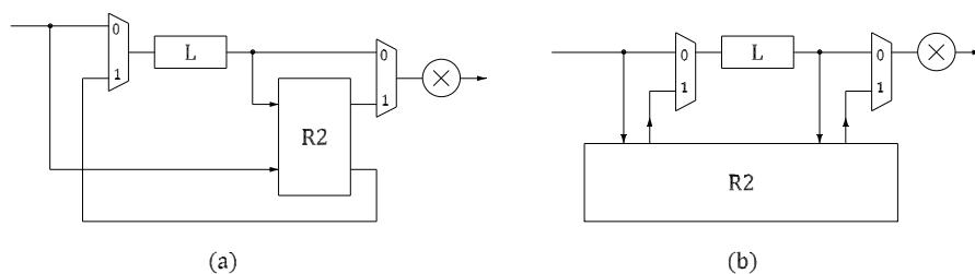
Fig. 8: Stage of a radix-2 SDF FFT architecture. (a) Conventional drawing. (b) Alternative drawing.
