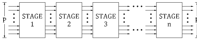
Fig. 6: Structure of a pipeline FFT architecture.
