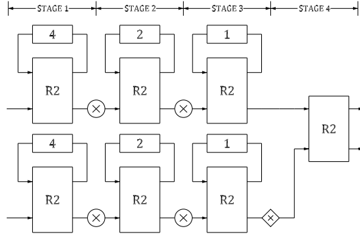
Fig. 30: 16-point 2-parallel radix-2 MDF FFT architecture.
