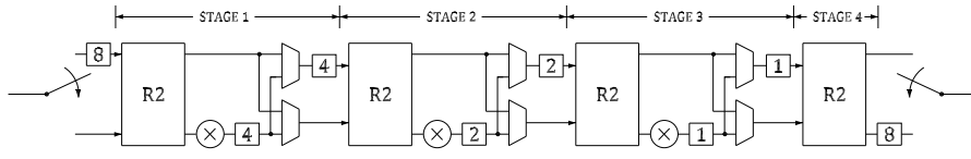
Fig. 19: 16-point radix-2 SDC FFT architecture.
