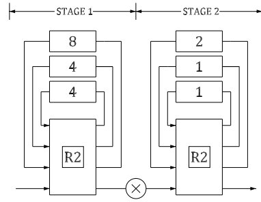
Fig. 14: 16-point deep feedback radix-2 SDF FFT architecture.
