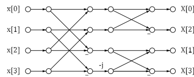
Fig. 4: Radix-4 butterfly.
