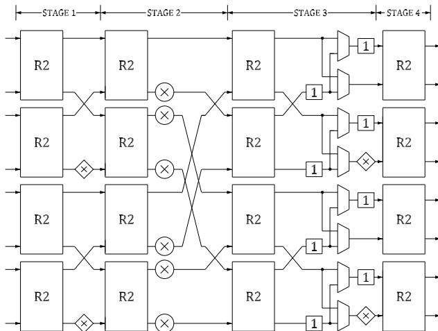
Fig. 42: 16-point 8-parallel radix- 2^2 MDC FFT architecture.
