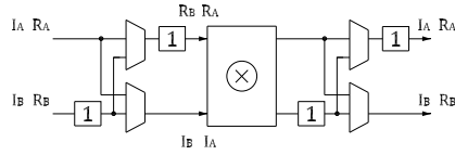
Fig. 22: Rotator in an SDC FFT architecture that divides the data in real and imaginary parts.
