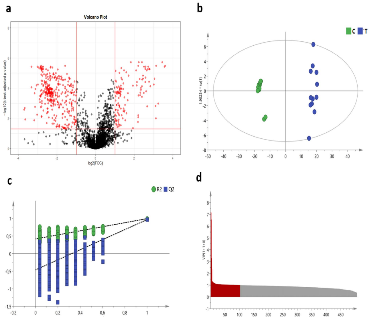
Figure 5. Fecal metabolome analysis. (a) Volcano plot; (b) OPLS-DA score plot (C: C group, T: T group); (c) permutation test plot ( R^2 : model fit of principal component analysis, Q^2 : predictive ability of the model); (d) Features with Variable Importance in the Projection > 1 (in red).
