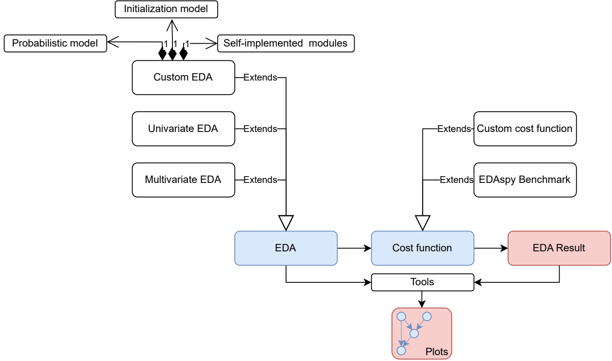
Figure 12.1: High order organization of the EDAspy library.
