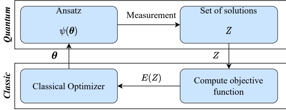
Figure 4.4: VQA workflow where, iteratively, the classical optimizer proposes a new set of parameters ( \theta ) for the ansatz \psi(\theta) , which is then measured ( Z ), and the objective function is computed ( E(Z) ).
