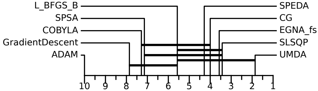
Figure 10.5: Critical difference diagram for the QAOA ansatz parameter tuning in terms of expectation value minimization comparing the different optimizers including the EDA variants.
