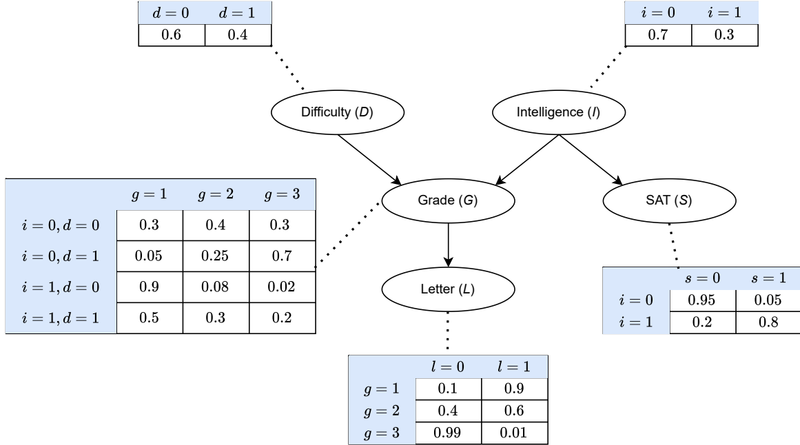
Figure 2.1: Student BN in which nodes are the variables of the problem, arcs represent conditional dependencies between the variables, and the tables are the CPDs.
