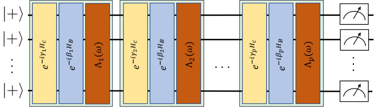
Figure 9.6: A quantum parametric circuit with p layers and 2p parameters. The initial state is a superposition of all the possible computational states, and after applying the p layers, a measurement along the Z axis of all the qubits is performed. Each layer is composed by the noise channel and both the cost and mixed operators.
