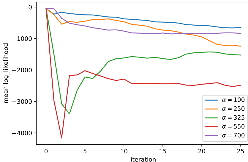
Figure 6.6: Mean log-likelihood of the set of solutions in each iteration along the optimization process for different values of \alpha parameter.
