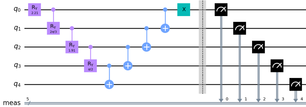
Figure 8.2: Example of a W state circuit for n = 5 . The probabilities are set to [\frac{1}{5}, \frac{1}{5}, \frac{1}{5}, \frac{1}{5}, \frac{1}{5}] . Purple gates are RY and CRY gates, blue ones are CX gates, green one is X gate, and black ones are the measurement gates.
