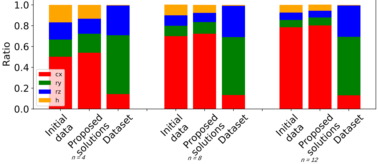
Figure 11.7: Ratio of \{CNOT, RY, RZ, H\} gates in the ansatz design of the randomly generated initial data ( G_0 ), best EDA solutions found ( EDA_i^n ), and dataset ( D_i^n ) [Nakayama et al., 2023], for n \in \{4, 8, 12\} , respectively.
