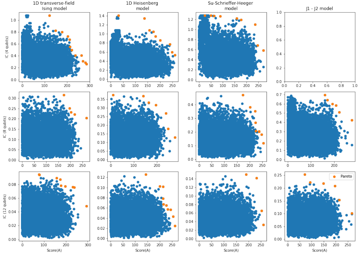
Figure E.1: Pareto frontier approximation (orange spots) over all the ansatz considered (blue spots) during optimization process. Columns refer to problem instances, while rows refer to number of qubits ( n ).
