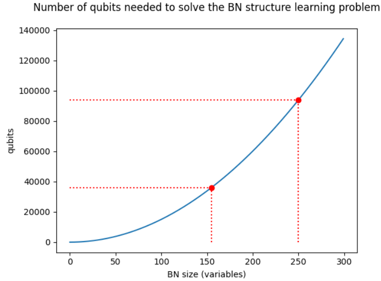
Figure D.1: In horizontal axis, the number of nodes, and in y axis, the number of quantum/classical bits needed for the QUBO formulation.
