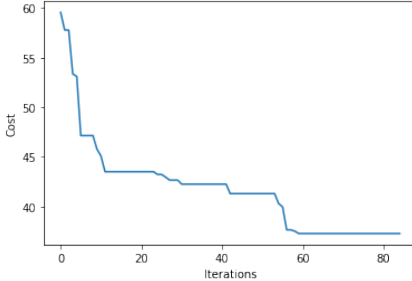
Figure 5.3: Best cost (Equation 5.1) found in each iteration of an EDA execution for a specific substance with restrictions.
