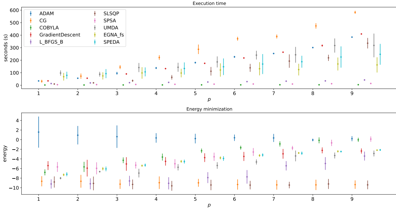
Figure 10.7: Comparison of the different EDA variants with the other state-of-the-art optimizers for the VQE TwoLocal ansatz parameter tuning. The top panel shows the mean computation time and standard deviation after running each algorithm 25 independent times for different number of layers p \in \{1, \dots, 9\} . The bottom panel shows the mean best expectation value achieved (Equation 4.9) and standard deviation after running each algorithm 25 independent times for different number of layers p \in \{1, \dots, 9\} .
