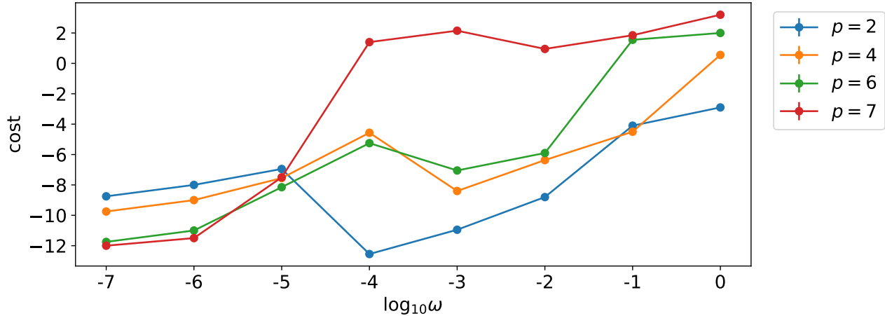
Figure 9.8: Mean best cost obtained for different values of the parameters \omega and p for 50 executions of the QAOA algorithm for the BNSL problem considering the amplitude damping error.
