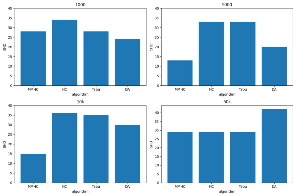
Figure D.2: Experiment for 20 nodes. Each subplot is a different size of dataset: 50000, 10000, 5000 and 1000 instances. DA is compared with the Hill Climbing algorithm (HC), Tabu search algorithm (Tabu), and Max-Min Hill Climbing algorithm (MMHC).
