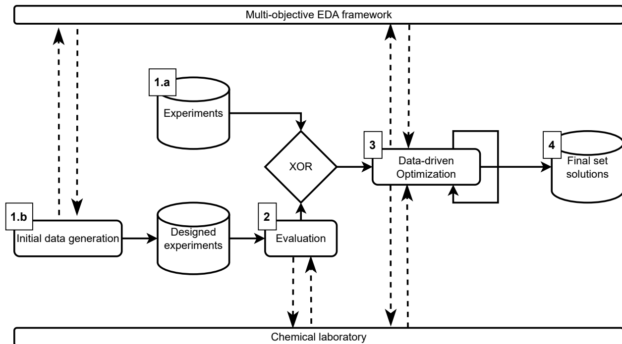
Figure 6.1: General flow chart of the multi-objective proposed approach for data-driven DoE.
