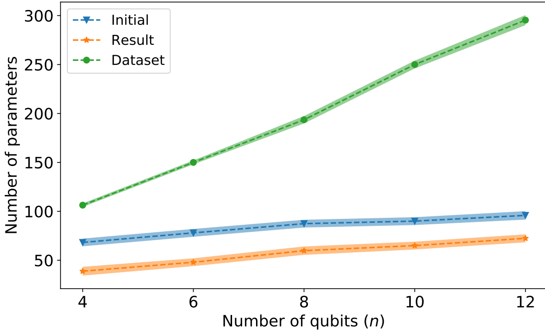
Figure 11.8: Mean and standard deviation of the number of parameters (Y-axis) as a function of the number of qubits (X-axis), in the ansatzes found in the randomly generated initial data ( G_0 ), best EDA solutions found (EDA _i^n ), and dataset ( D_i^n ) [Nakayama et al., 2023]. Note that the values for n = 6, 10 have been approximated through a linear regression.
