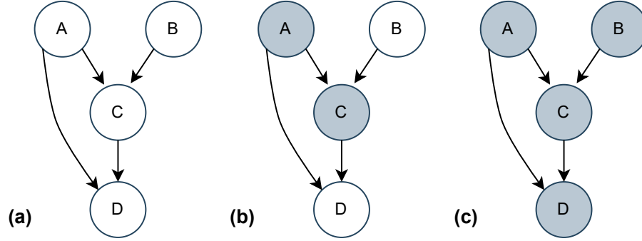
Figure 2.3: Parametric (a), semiparametric (b) and non-parametric (c) BN examples, where white nodes and grey nodes represent parametric and non-parametric conditional distributions, respectively.
