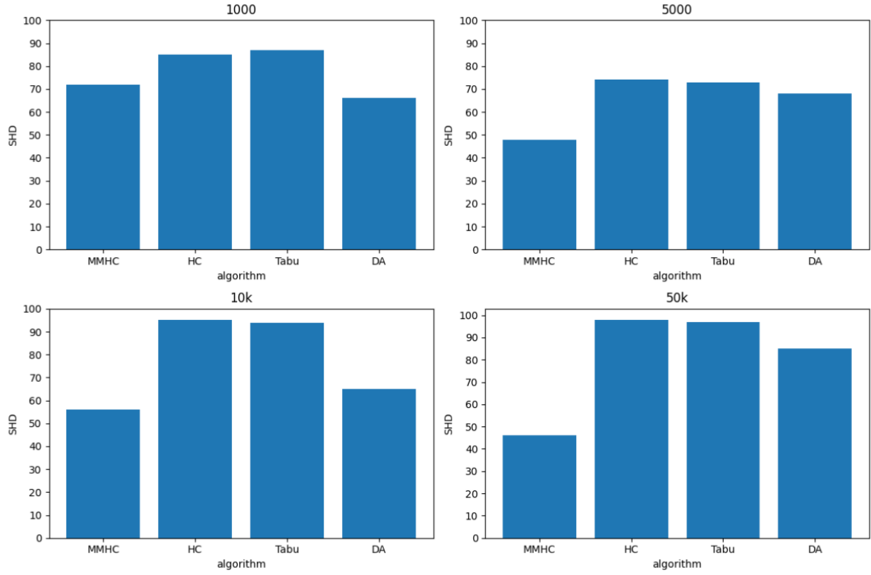
Figure D.3: Experiment for 50 nodes. Each subplot is a different size of dataset: 50000, 10000, 5000 and 1000 instances. DA is compared with the Hill Climbing algorithm (HC), Tabu search algorithm (Tabu), and Max-Min Hill Climbing algorithm (MMHC).
