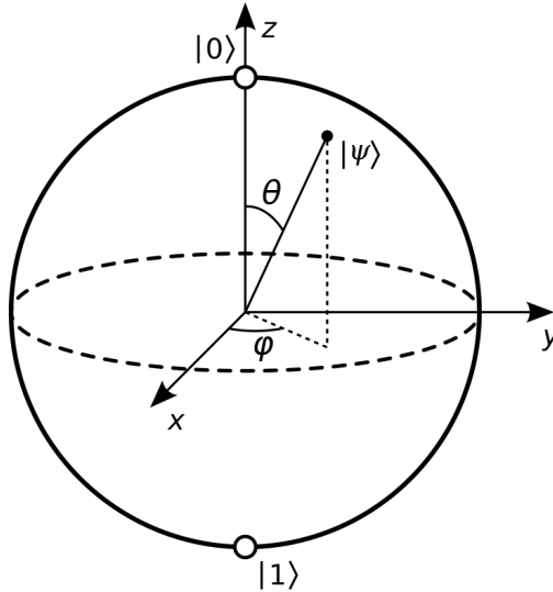
Figure 4.1: Bloch sphere representation of a qubit.
