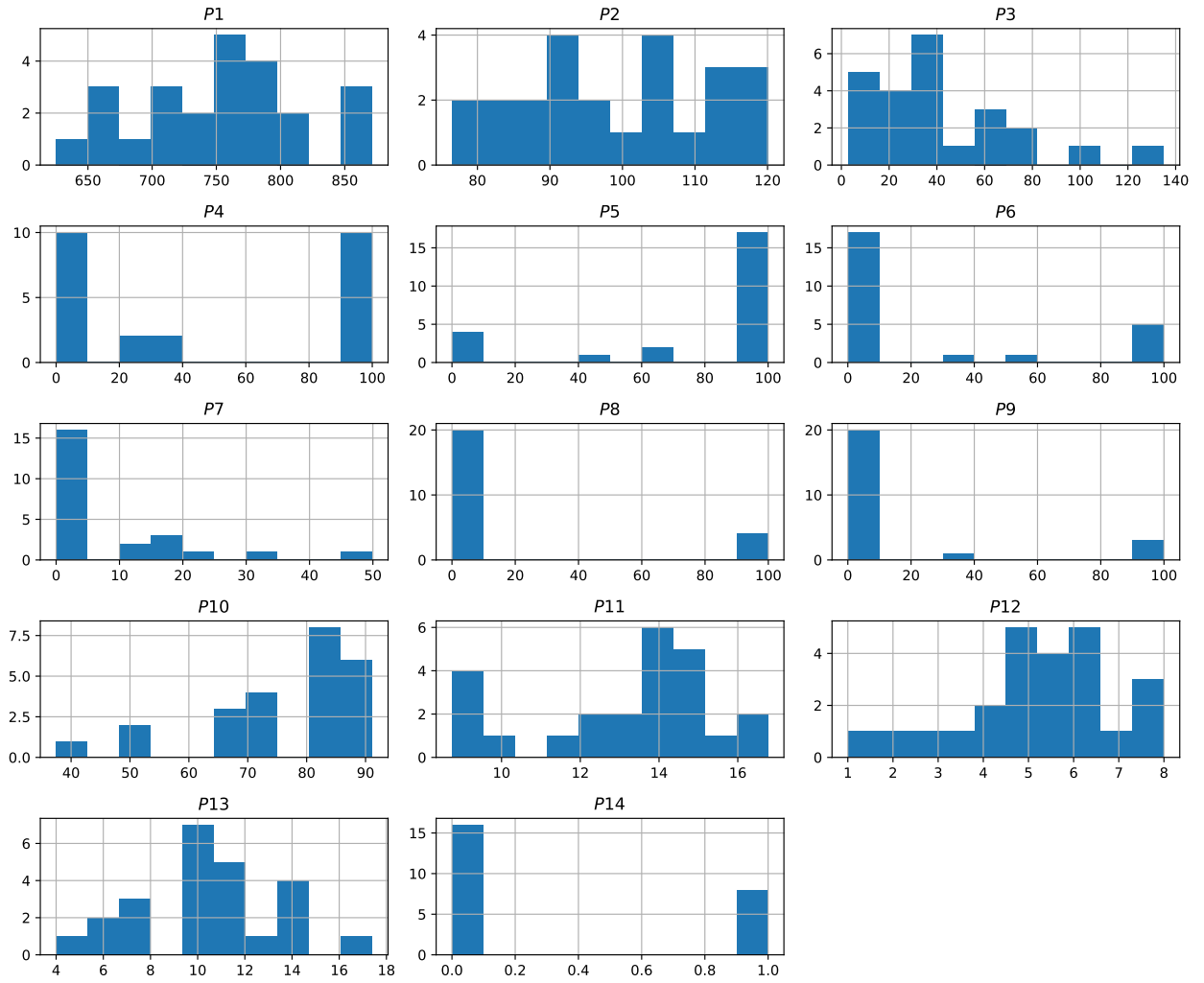
Figure B.1: Frequency of each property P_1, \dots, P_{14} .
