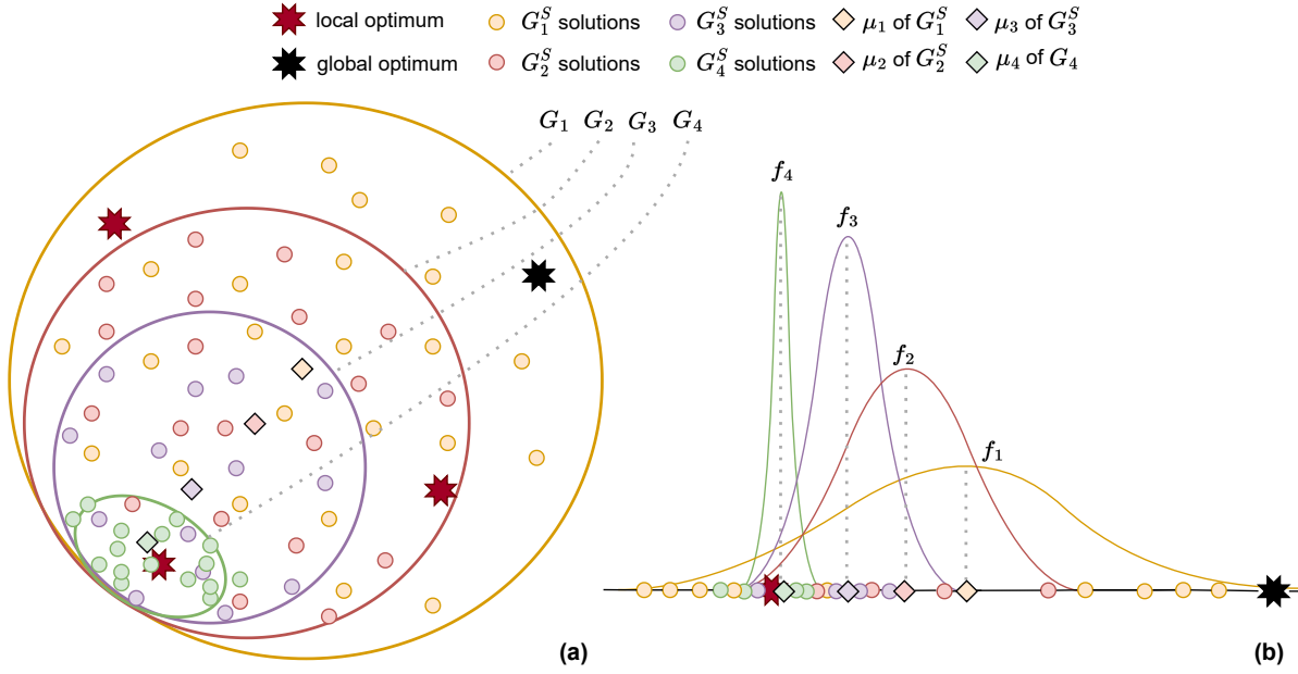
Figure 7.1: A search space that is iteratively approximated by an EGNA in two (a) and one (b) dimensions, where a single global optimum (black star) and some local optima (red stars) exist. The means and the search space area defined by the solutions of each generation G_t are represented by squares, and ellipses, respectively, in the two dimensional landscape and by squares and a Gaussian density function in the one dimensional landscape.
