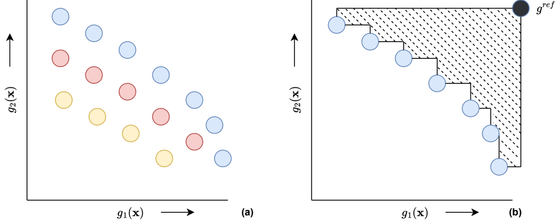
Figure 3.3: Panel (a) shows first, second and third Pareto frontiers represented as blue, red and yellow circles, respectively, for maximizing g_1(\mathbf{x}) and g_2(\mathbf{x}) objectives simultaneously. Panel (b) shows the hypervolume (HV) indicator computation for the first Pareto frontier and the reference point g^{ref} .
