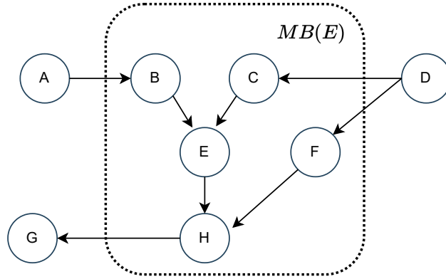
Figure 2.2: Illustrative example of the set of variables included in the Markov blanket of variable E , which includes the parents, children, and parents of children of E .
