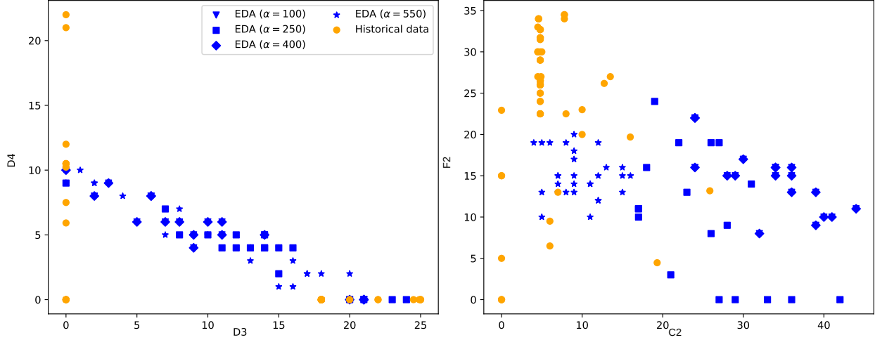
Figure 6.7: Comparison of two dimensions of the problem landscape where orange circles represent traditional formulas found in the historical data, and the rest of symbols represent the new optimal formulas found by the our approach. The left panel compares D4 and D3 ingredients and the right panel compares F2 and C2 ingredients.
