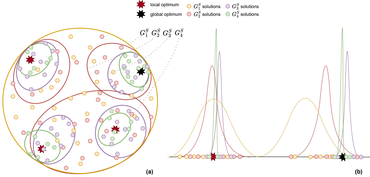
Figure 7.3: A search space iteratively approximated by SPEDA in two (a) and one (b) dimensions is shown, where a single global optimum (black star) and some local optima (red stars) exist. The search space area defined by the solutions of each generation G_t are represented by ellipses and a density function on the two and one dimensional landscapes, respectively.
