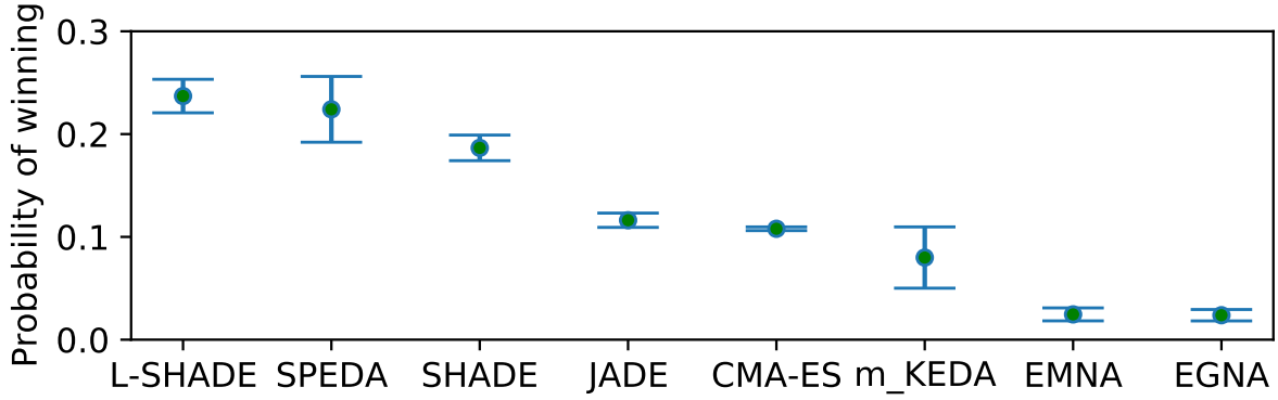
Figure 7.5: Credible intervals (5% and 95% quantiles) and expected probability of winning (green dots) for results shown in Table 7.2.
