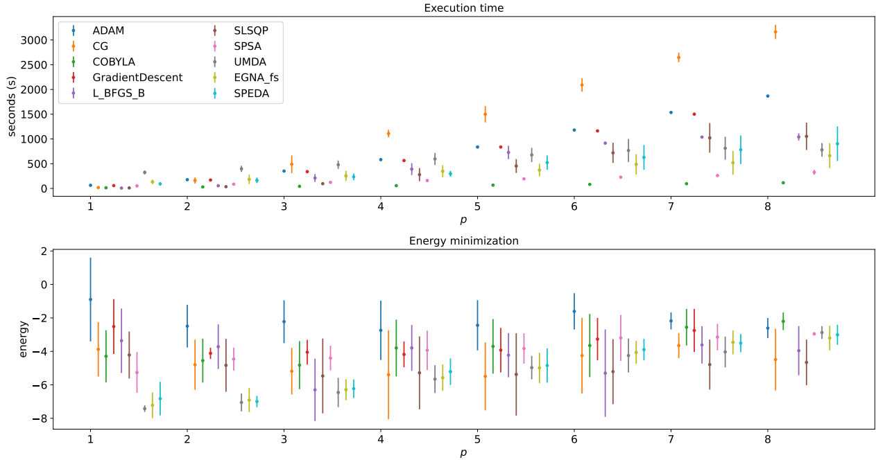
Figure 10.3: Comparison of the different EDA variants with the other state-of-the-art optimizers for the QAOA ansatz parameter tuning. The top panel shows the mean computation time and standard deviation after running each algorithm 25 independent times for different number of layers p \in \{1, \dots, 8\} . The bottom panel shows the mean best expectation value achieved (Equation 4.9) and standard deviation after running each algorithm 25 independent times for different number of layers p \in \{1, \dots, 8\} .
