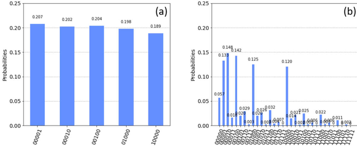
Figure 8.3: Probability distribution of the W state circuit sampling for n = 5 without (a) and with (b) noise. The quantum circuit was run 1000 times for each scenario.
