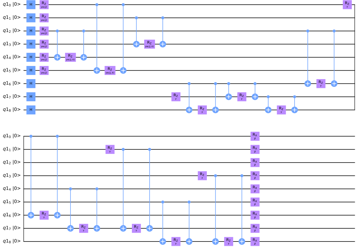
Figure 9.1: A QAOA circuit example for a BNSL problem with 3 nodes and 1 layer. This variational ansatz has \gamma and \beta parameters as the parameters of the first layer of the circuit.
