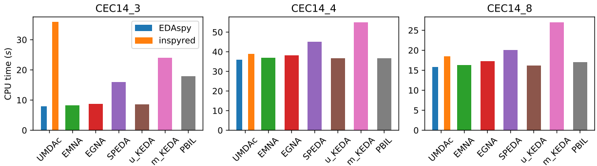
Figure 12.4: CPU runtime analysis of some EDA variants for continuous optimization. UMDA C , EMNA, EGNA, SPEDA, univariate KEDA (u_KEDA), multivariate KEDA (m_KEDA) and PBIL are shown.
