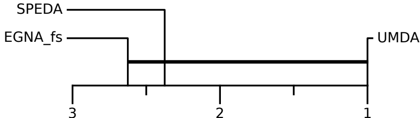
Figure 10.9: Critical difference diagram for the VQE TwoLocal ansatz parameter tuning ( p \geq 6 ) in terms of expectation value minimization using the three EDA variants.
