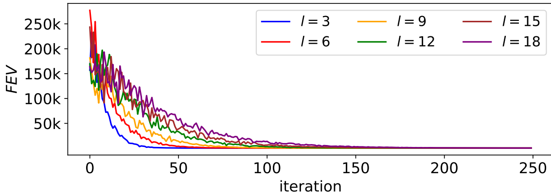
Figure 7.7: Mean best cost found ( FEV ) by SPEDA for the cec14_3 for different archive lengths ( l ) during runtime after executing each experiment 25 independent times.
