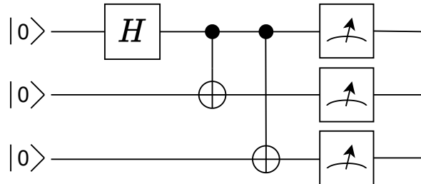
Figure 4.3: GHZ quantum circuit.
