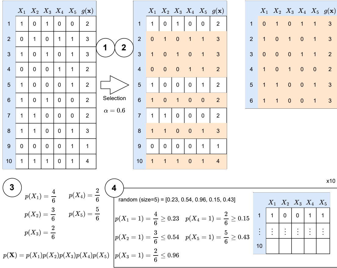
Figure 3.1: Toy example of EDA for the OneMax optimization problem.
