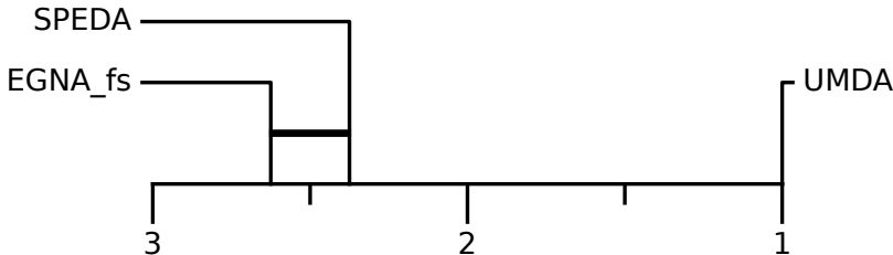
Figure 10.8: Critical difference diagram for the VQE TwoLocal ansatz parameter tuning in terms of expectation value minimization using three EDA variants.
