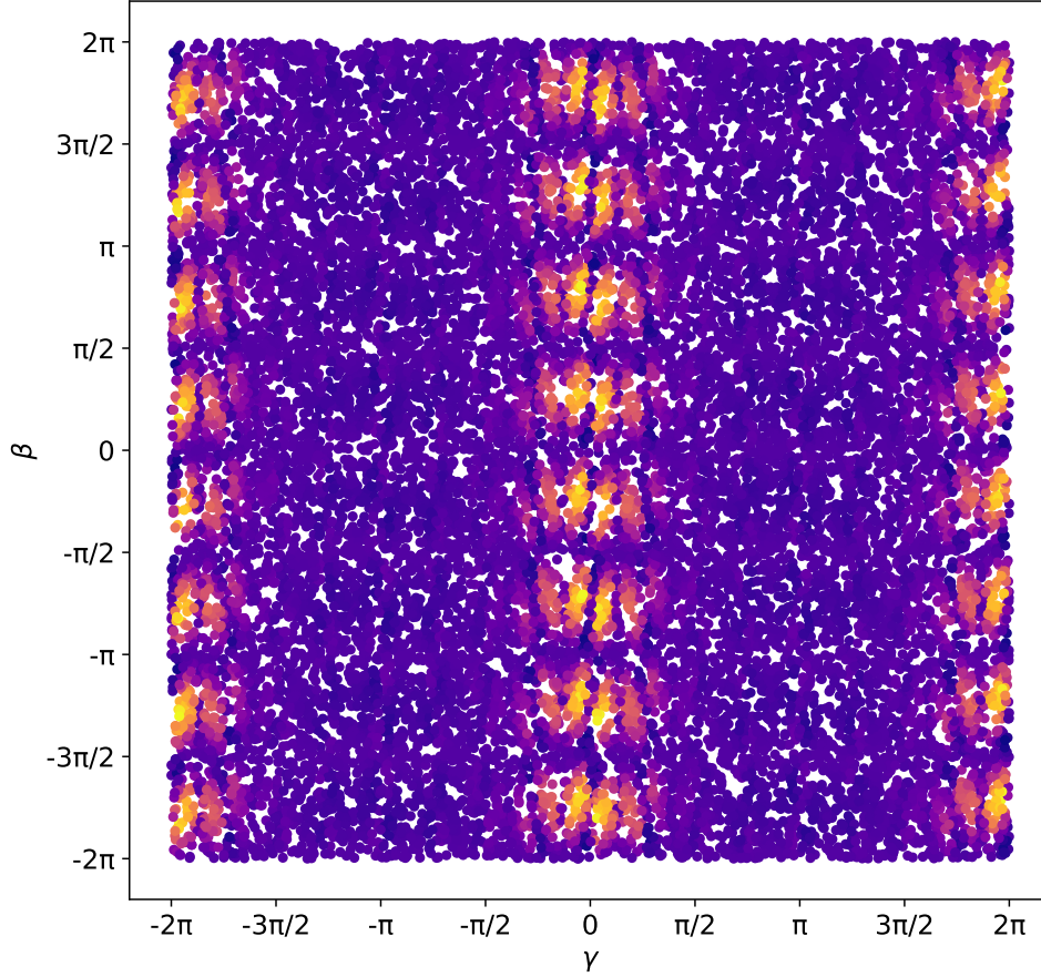
Figure 10.1: Optimization landscape where Y - and X -axis represent, respectively, \beta and \gamma QAOA ansatz parameters for p = 1 layer, and the lighted regions over the purple background represent the optimum parameters that minimize the expectation value (Equation 4.9). Although the parameter tuning has been restricted to \theta \in [0, 2\pi]^n , the landscape of \theta \in [-2\pi, 2\pi]^n is displayed to show that -2\pi is equivalent to 2\pi .
