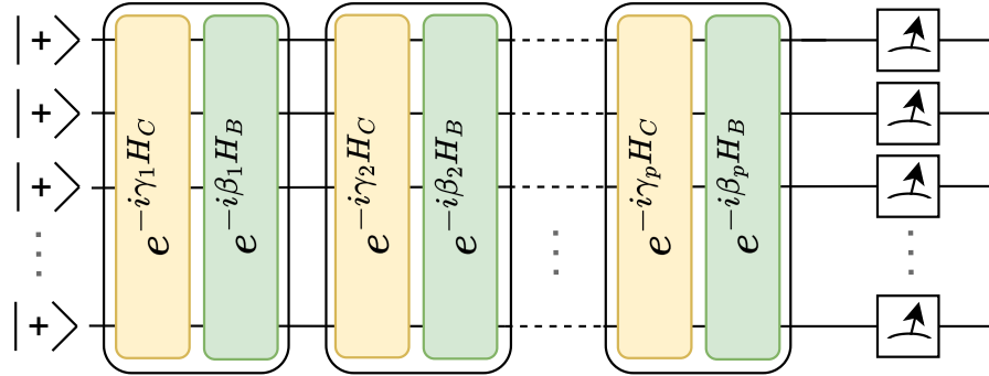
Figure 4.5: An ansatz with p layers and 2p parameters to be tuned. The quantum circuit starts from a superposition state over all the possible computational states, then applies p layers, and measures the qubits in the Z -axis.
