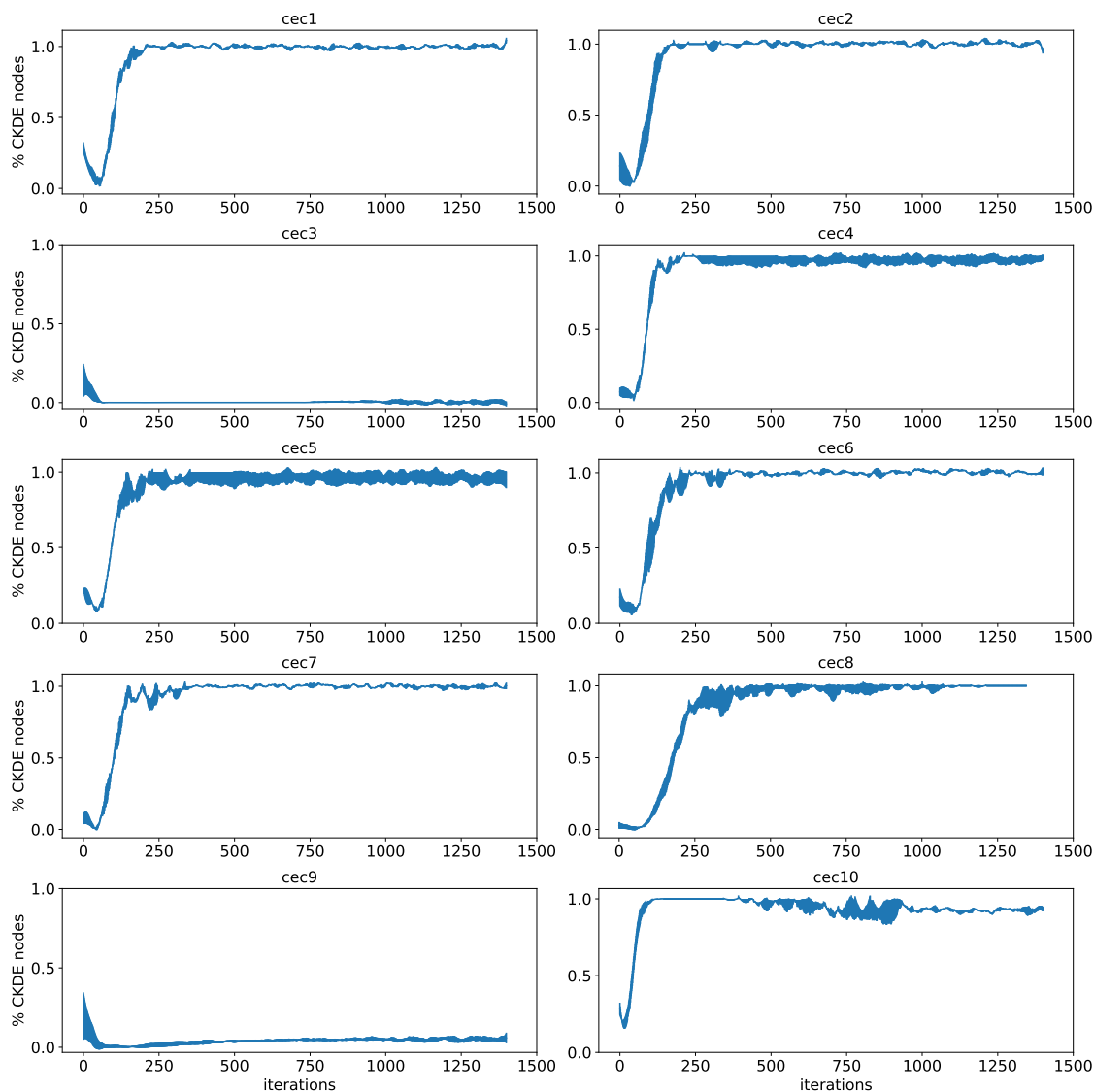
Figure 7.4: Percentage of CKDE nodes during runtime, mean and standard deviation of 25 independent executions. The experimental results for the first 10 benchmarks are shown with d = 30 .
