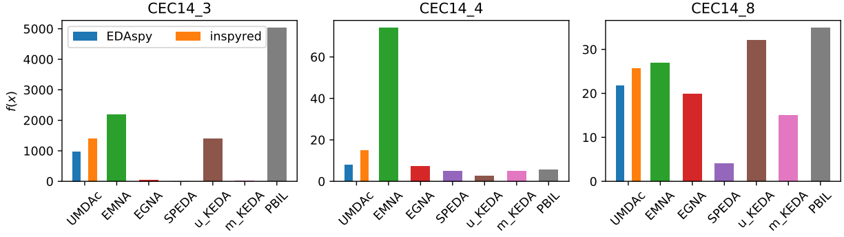
Figure 12.3: Best cost found analysis of some EDA variants for continuous optimization. UMDA C , EMNA, EGNA, SPEDA, univariate KEDA (u_KEDA), multivariate KEDA (m_KEDA) and PBIL are shown.
