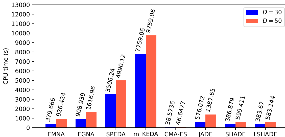
Figure 7.10: Comparison of the average CPU time (in seconds) after 25 independent executions on each of the benchmarks in CEC2014 and CEC2017, for EMNA, EGNA, m_KEDA, SPEDA, CMA-ES, JADE, SHADE and LSHADE. The results for 30 and 50 dimensions are shown in blue and red, respectively.
