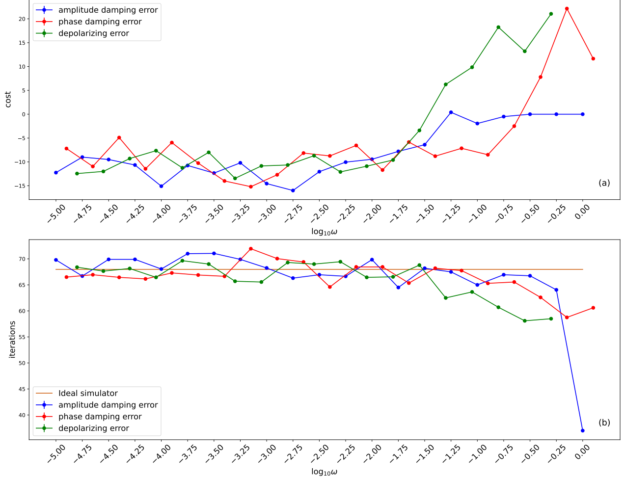
Figure 9.7: Mean best costs (a) and mean numbers of iterations until convergence (b) as a function of the noise amplitude \omega . Blue, red and green lines represent the simulated amplitude, phase damping and depolarizing noise models, respectively. For the detailed mean and standard deviation values of these experiments, see Table 9.1. Fifty different executions of the QAOA algorithm were run for the 4 node BNSL problem, and p = 3 .
