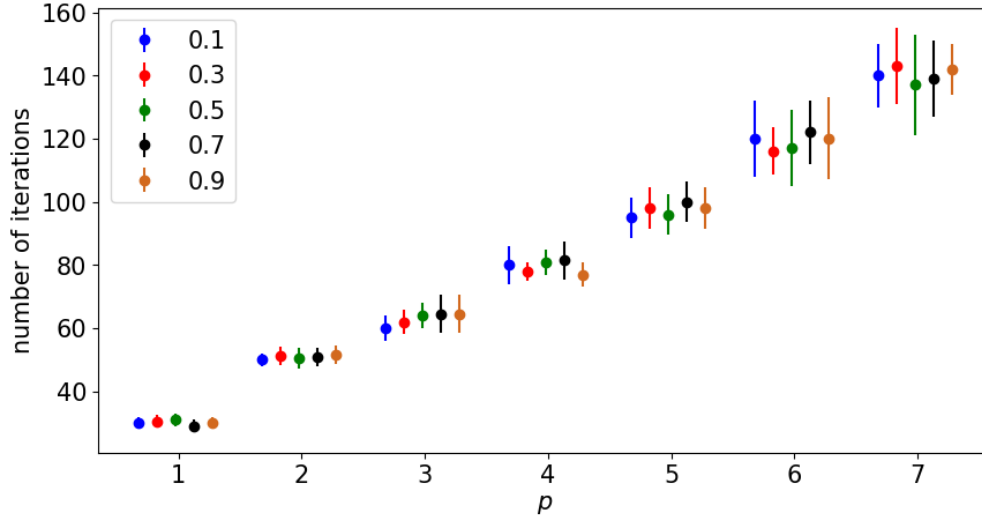
Figure 9.5: Means and standard deviations of the number of iterations until convergence after executing the QAOA 50 times for different values of p (X-axis) and \alpha (colours).
