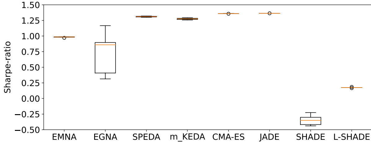
Figure 7.9: Boxplot with the best results found by each algorithm after 25 independent executions for the specific portfolio optimization problem.
