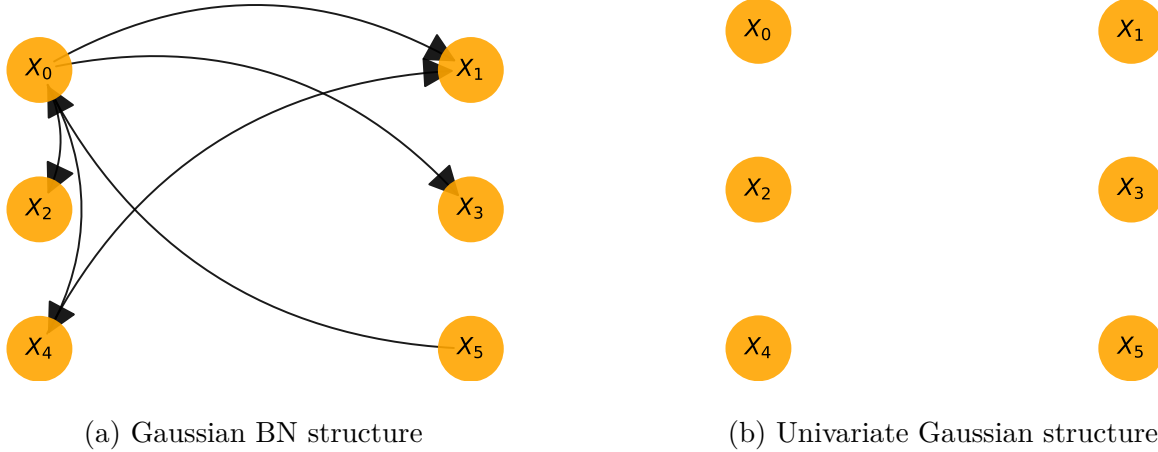
Figure 12.2: Probabilistic models graphical representations.
