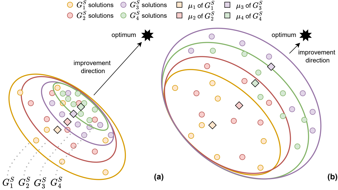
Figure 7.2: Two search processes are shown in which each generation G_t is obtained by sampling a probabilistic model estimated (a) from the best individuals of the previous generation or (b) from the best individuals of the previous l generations. The means and the search area defined by the solutions of each generation G_t are represented by squares and ellipses, respectively, on the two dimensional landscape.
