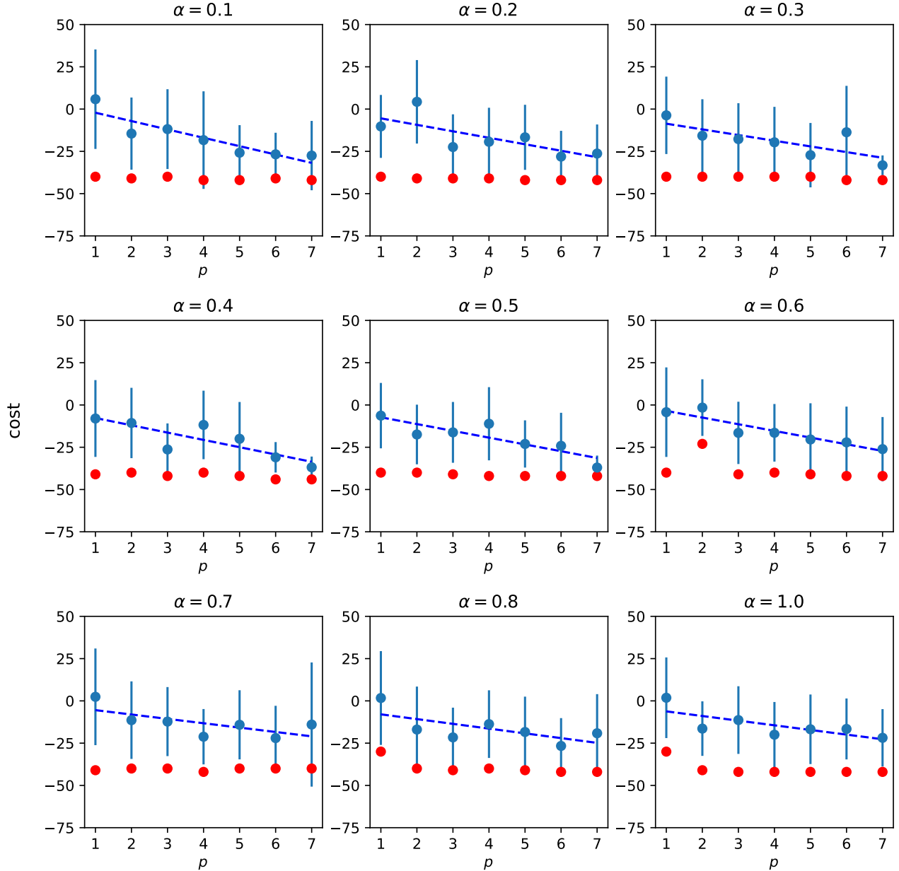
Figure 9.4: Minimization of the \text{CVaR}(\alpha) (Equation 4.11) for different numbers of layers p (X-axis) in the QAOA circuit and different values of the parameter \alpha . Blue dots and error bars correspond to the means and standard deviations of the best results found after executing the QAOA 50 times, respectively, and red denotes the minimum costs found in those executions. Dashed trend lines are plotted to guide the human eye.
