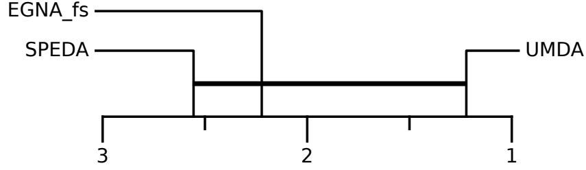
Figure 10.4: Critical difference diagram using Friedman tests to reject the null hypothesis of equal expected value, and a post-hoc analysis based on the Wilcoxon-Holm method. The horizontal black line connects the EDA variants that do not have a significant difference in the QAOA ansatz parameter tuning in terms of expectation value minimization using the three EDA variants.
