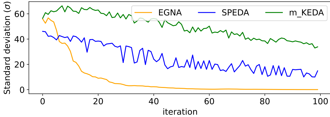
Figure 7.6: Mean standard deviation (Y-axis) between the best solutions in the same iteration during runtime (X-axis) after executing EGNA, SPEDA and m_KEDA approaches 25 independent times, for the cec14_4 benchmark ( d = 30 ). Note that this plot represents one variable out of d .
