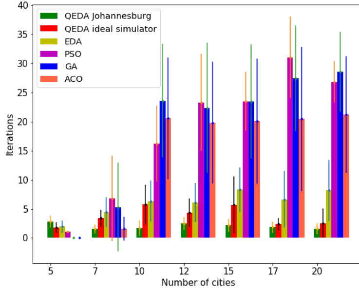
Figure 8.5: Mean convergence for the TSP for different number of cities and different algorithms: QIEDA executed in the Johannesburg quantum simulator with noise, QIEDA executed in a quantum simulator without quantum noise, the non-quantum estimation of distribution algorithm (EDA), particle swarm optimization (PSO), GA, and the ant colony optimization (ACO).
