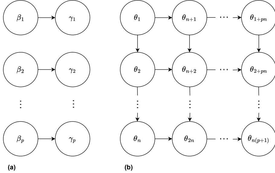
Figure 10.2: GBN structures designed for QAOA (a) and VQE TwoLocal (b) ansatz parameter tuning embedded by EGNA. Each node represents a parameter in the ansatz , and an arc between two nodes represents a linear Gaussian dependency between both variables.
