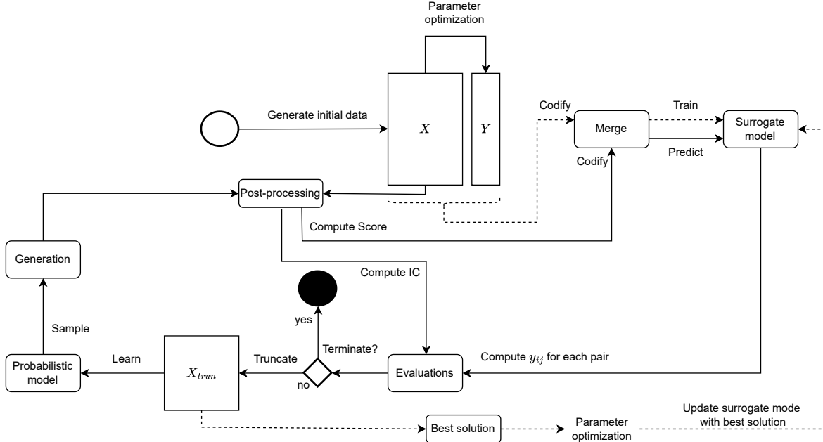
Figure 11.1: Flowchart of the proposed approach, starting from the white spot and finishing in the black spot one the convergence criteria is met. Dashed lines regard the train and update of the surrogate model.
