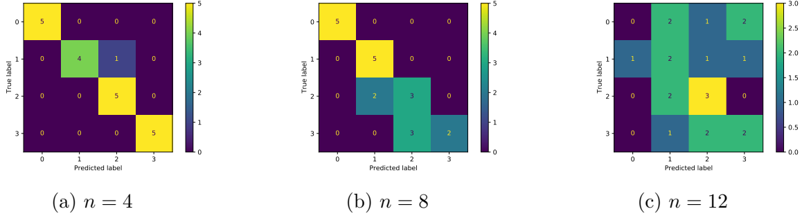
Figure 11.5: Confusion matrices for n \in \{4, 8, 12\} .
