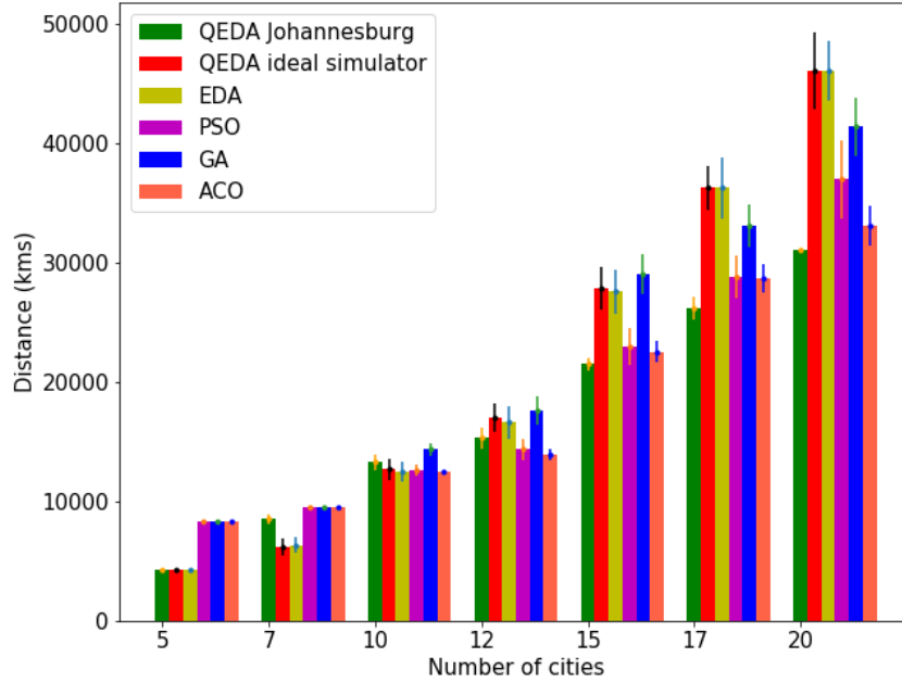
Figure 8.4: Mean best cost for the TSP for different number of cities and different algorithms: QIEDA executed in the Johannesburg quantum simulator with noise, QIEDA executed in a quantum simulator without quantum noise, the non-quantum estimation of distribution algorithm (EDA), particle swarm optimization (PSO), GA, and the ant colony optimization (ACO).
