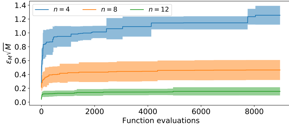
Figure 11.6: Mean and standard deviation of IC maximization aggregating the optimization process of different H_i for different numbers of qubits ( n ).
