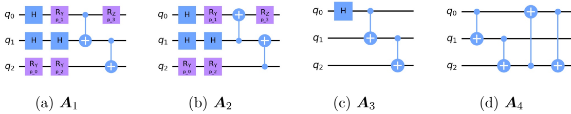
Figure 11.2: Four examples of the ansatz codifications ( \mathbf{A}_1 , \mathbf{A}_2 , \mathbf{A}_3 , \mathbf{A}_4 ) defined in Equation 11.2
