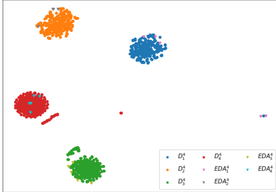
Figure 11.4: Visualization of the ansatzes found in the dataset ( D_i^n ) using t-SNE [Van der Maaten and Hinton, 2008], which are colored depending on the Hamiltonian to be solved ( H_i , where i \in \{1, 2, 3, 4\} ). Additionally, the best architectures found by the EDA approach ( EDA_i^n ) are represented using different colored and shaped points. Note that EDA_i^n regards the solutions found for Hamiltonian H_i . All the results shown correspond to n = 4 .
