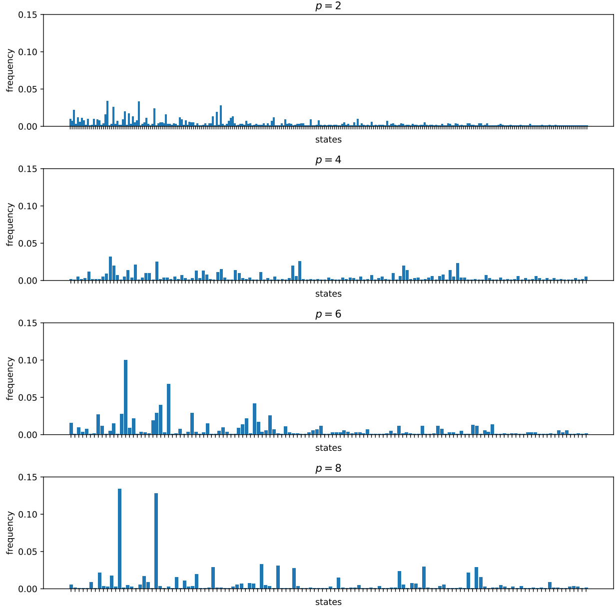
Figure 9.3: Histograms for different numbers of layers p for the same BNSL problem. The Y and X axes represent the frequency, and the solutions, respectively. The names of the solutions have been removed from the X -axis for aesthetics, but how they are sorted is the same for each subplot.
