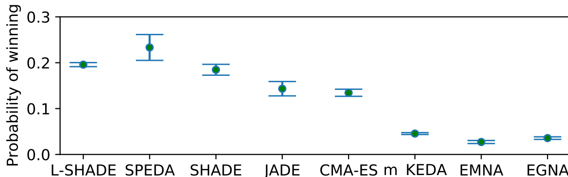
Figure 7.8: Credible intervals (5% and 95% quantiles) and expected probability of winning (green dots) for results shown in Table 7.3.
