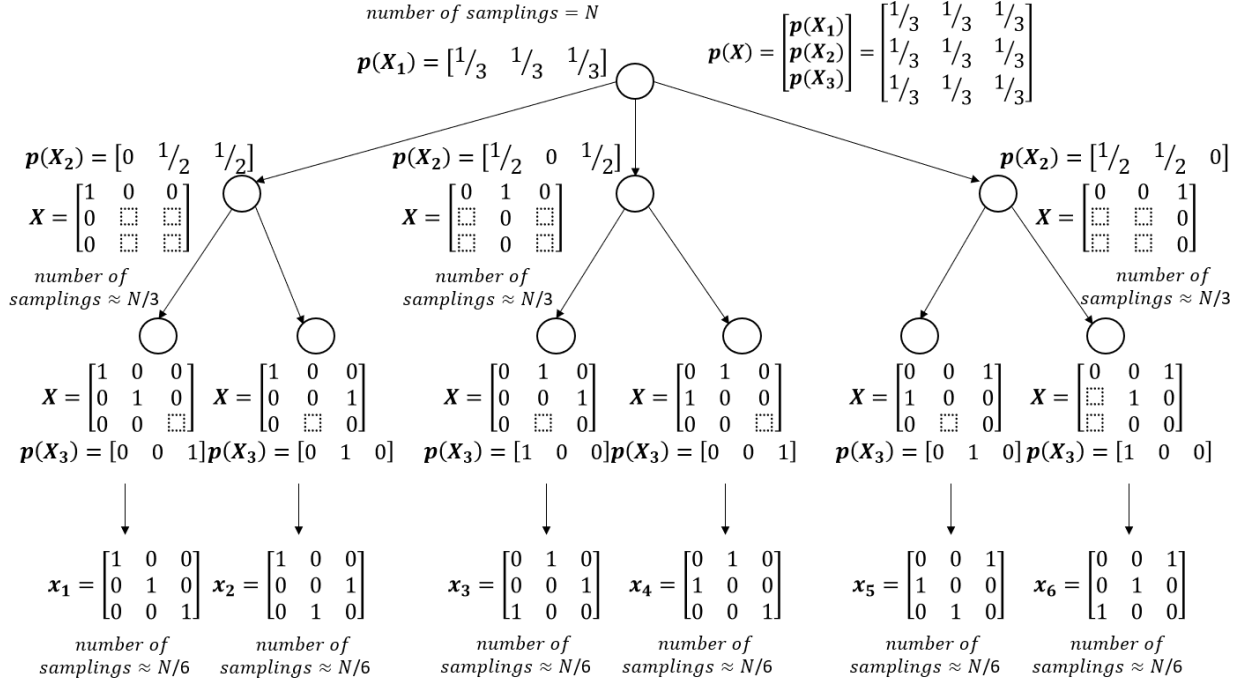
Figure 8.1: Example of the quantum individuals sampling of size n = 3 . An initial matrix of statistics p(\mathbf{X}) is updated in each node depending on its parents samplings. In the leaf nodes, the final individuals are obtained. The algorithm samples N individuals. Each node distributes its number of samples among its child nodes.
