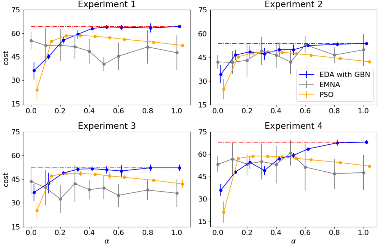
Figure 5.7: Mean cost and standard deviation of EDA with a Gaussian Bayesian network, and the EMNA and PSO algorithms as a function of the \alpha parameter (Equation 5.2) for the different experiments. For each value of \alpha , 20 simulations were run. The dashed line corresponds to the cost of solvents traditionally used in the laboratory processes for this specific substance and set of restrictions.
