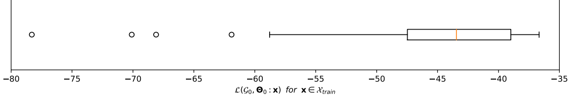
Figure 6.2: Box plot of the log-likelihood of each sample from \mathcal{X}_{train} in the model represented as (\mathcal{G}_0, \Theta_0) , where mean and median are approximately -46 and -42, respectively.
