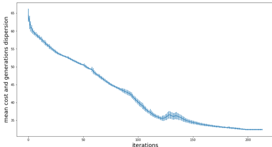
Figure 5.4: Mean cost (Equation 5.1) and dispersion among individuals in each generation for a specific substance with restrictions.
