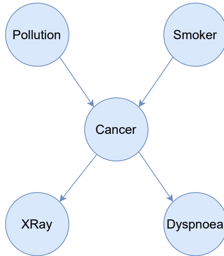
Figure 9.9: Original Cancer BN structure composed of 5 nodes that represent 5 discrete variables and 4 arcs.
