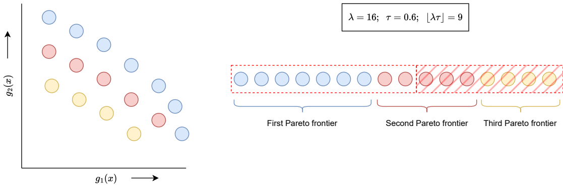
Figure 6.3: First, second and third Pareto frontiers represented as blue, red and yellow circles, respectively, are identified for maximizing g_1(\mathbf{x}) and g_2(\mathbf{x}) objectives, and ranked for the truncation process. An example for N = 16 and \tau = 0.6 is shown.
