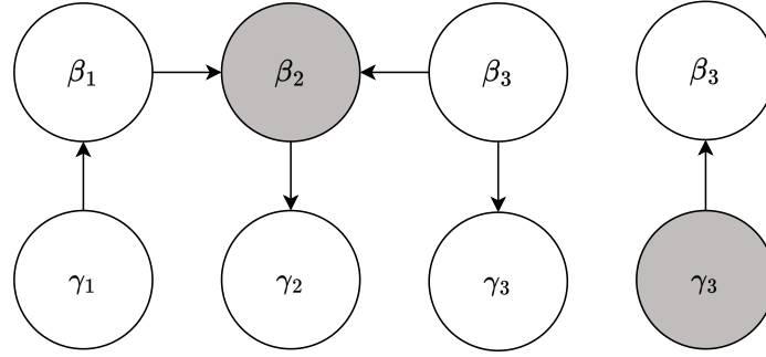
Figure 10.6: BN structure where the common arcs found in the BNs of the last iterations of 10 different SPEDA runs for the QAOA ansatz parameter tuning with p = 4 are represented. White and grey nodes represent the Gaussian and KDE nodes, respectively.
