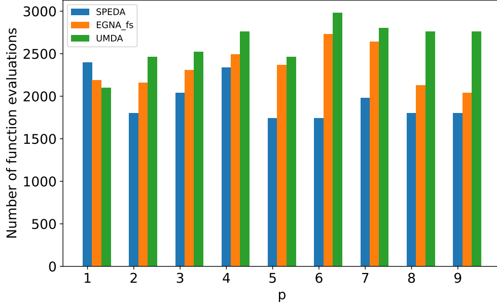
Figure 10.10: Comparison of the mean number of cost function evaluations for the VQE TwoLocal ansatz parameter tuning after executing each EDA variant 25 independent times. Each cost function evaluation involves a new ansatz parameter configuration and measuring the quantum circuit N times.
