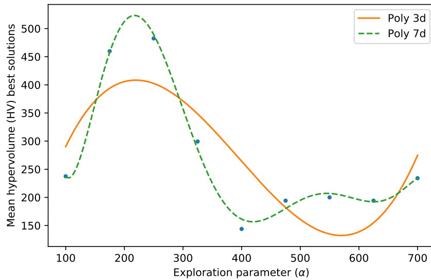
Figure 6.5: Mean HV after running the EDA approach 25 independent times for different values of exploratory parameter \alpha . Blue dots represent the HV mean values, and orange and green dashed lines represent a function approximation using a polynomial with degree three and seven, respectively.
