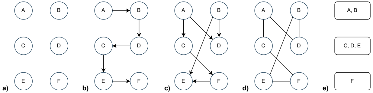
Figure 3.2: Examples of different types of PM structures used in EDAs.
