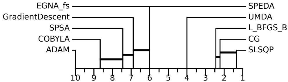
Figure 10.11: Critical difference diagram for the VQE TwoLocal ansatz parameter tuning in terms of expectation value minimization comparing the different optimizers including the EDA variants.
