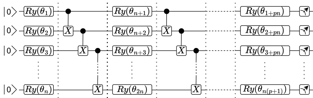
Figure 4.6: TwoLocal ansatz used for the VQE with p \in \mathbb{N} layers, n qubits and pn parameters. Each layer applied a rotation gate in the Y -axis over each qubit. Between each layer, a linear entanglement is applied in the system, where each qubit i is connected through a two-qubit rotation gate in the X -axis to the qubit i + 1 .
