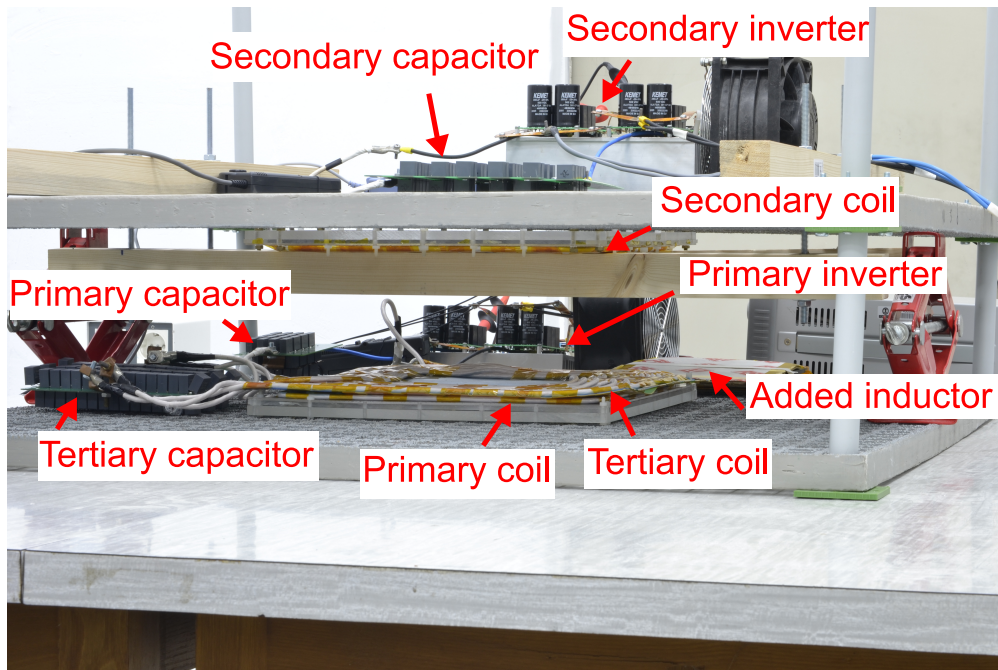
Figure 3.11: Experimental setup
