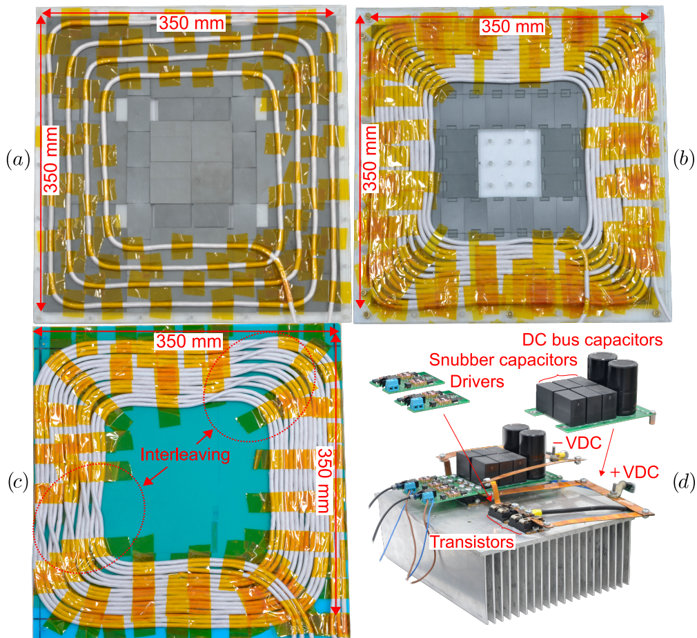
Figure 3.12: a) Primary coil b) Secondary coil c) Tertiary coil d) Inverter
