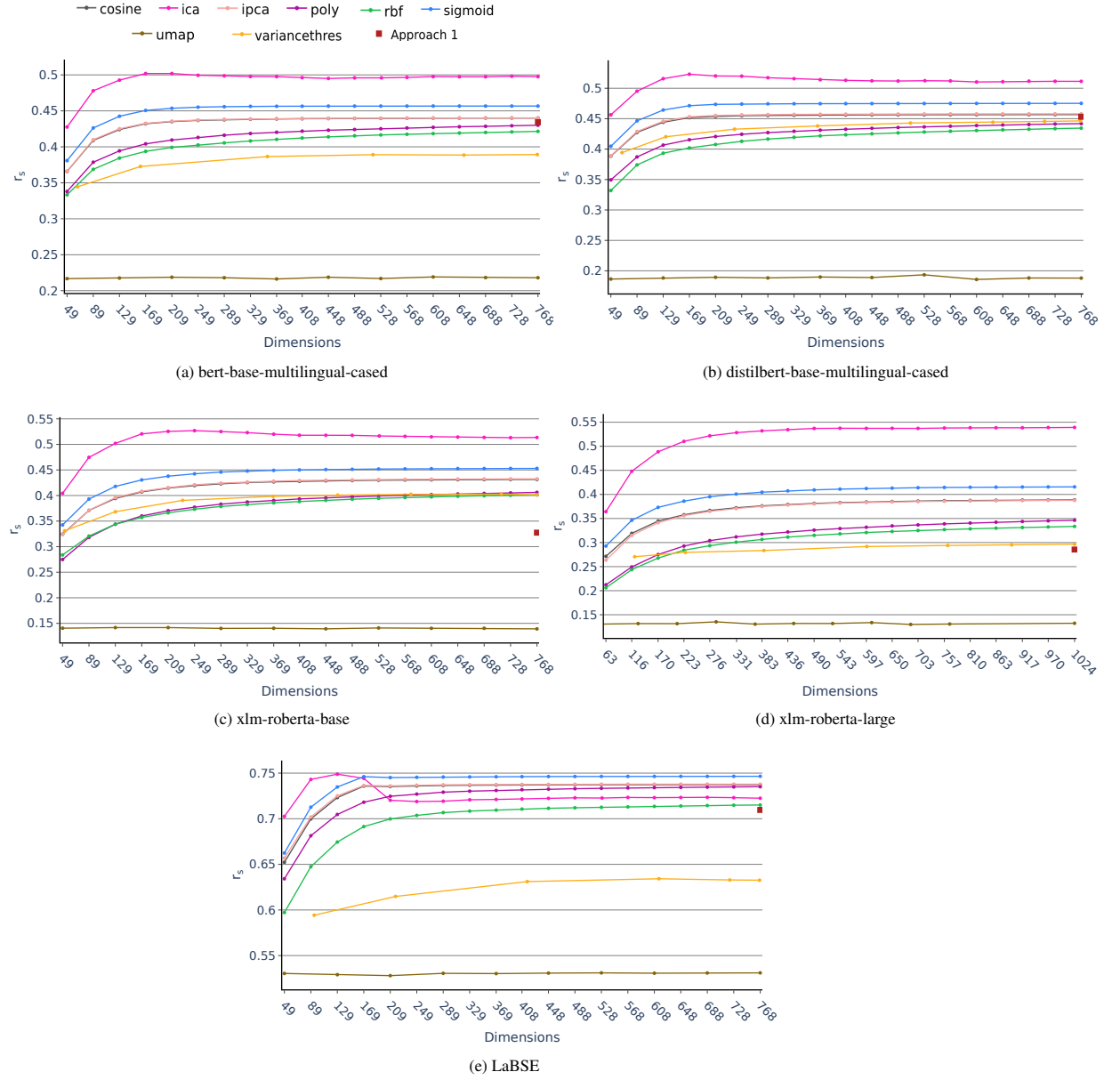
Figure 3: Approach 3 average Spearman r_s correlation coefficient in multilingual tasks from the mSTSb test as a function of the number of dimension for the different dimensionality reduction techniques grouped by model.
