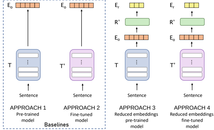
Figure 1: Representation of the approaches followed to evaluate the impact of different dimensionality reduction techniques in multilingual transformers. Where T represents the pre-trained transformer model, T' the fine-tuned transformer model, R' the fitted dimensionality reduction technique, E_o the original output embedding, and E_r the reduced embedding.
