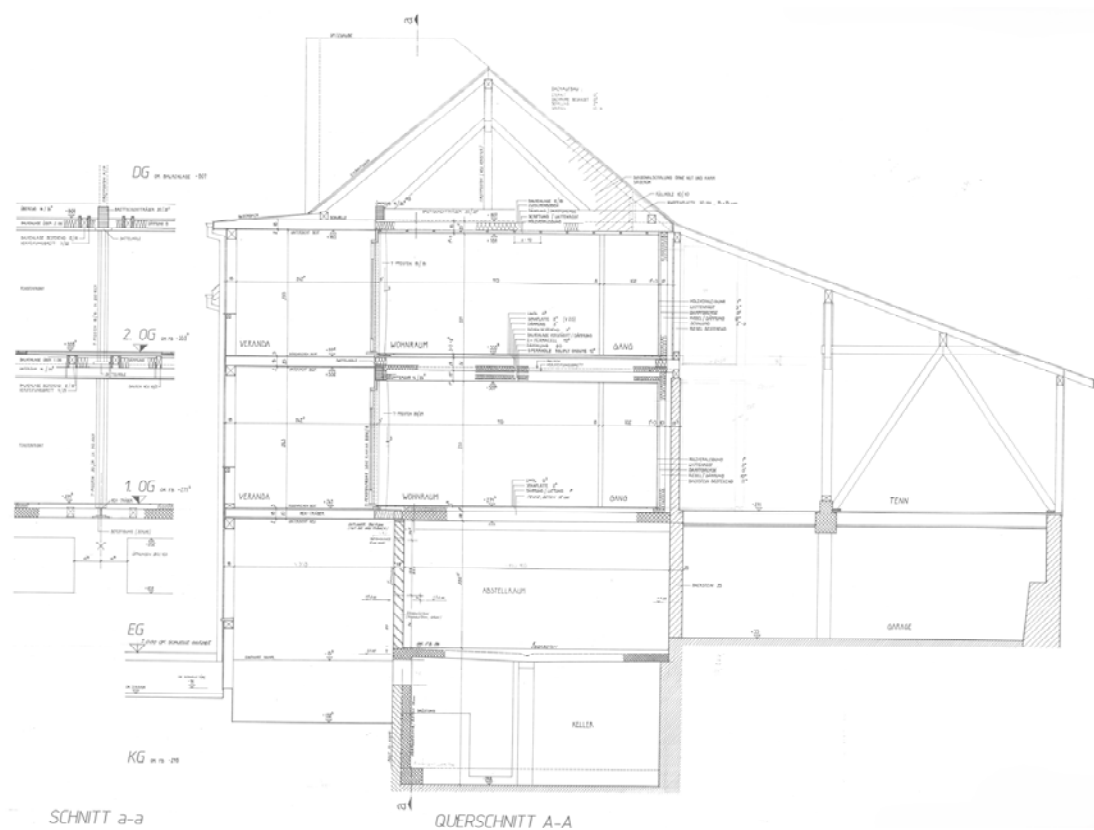
Figure 21. Walenstadtberg Housing. The construction cross section of the project (1992). Note the entasis of the pillars, the reduction in their section between the first and second floors, and the detail of the reinforcement of the wooden slabs on the left. The southwest façade of the first floor is aligned with that of the second floor (originally it was aligned with the ground floor). Material provided by Gody Kühnis.
