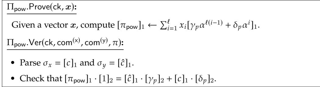
Figure 5.2: Power type chaining proof \Pi_{\text{pow}} .
