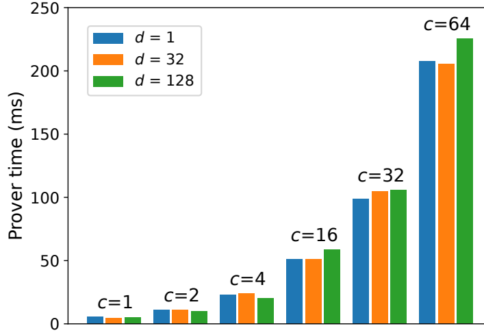
Figure 8.8: Prover time for varying number of channels c , d and fixed n = 64 and m = 4 .
