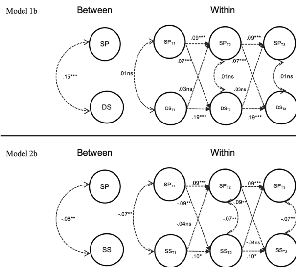
Figure 1. Standardized Parameter Estimates for the RI-CLPM Models 1b and 2b ( N = 1,878 ).
