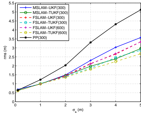
Figure 7 – RMS position error for the targets with one target (target two in Fig. 4). FSLAM-TUKF provides a slightly better estimate than MSLAM-TUKF.
