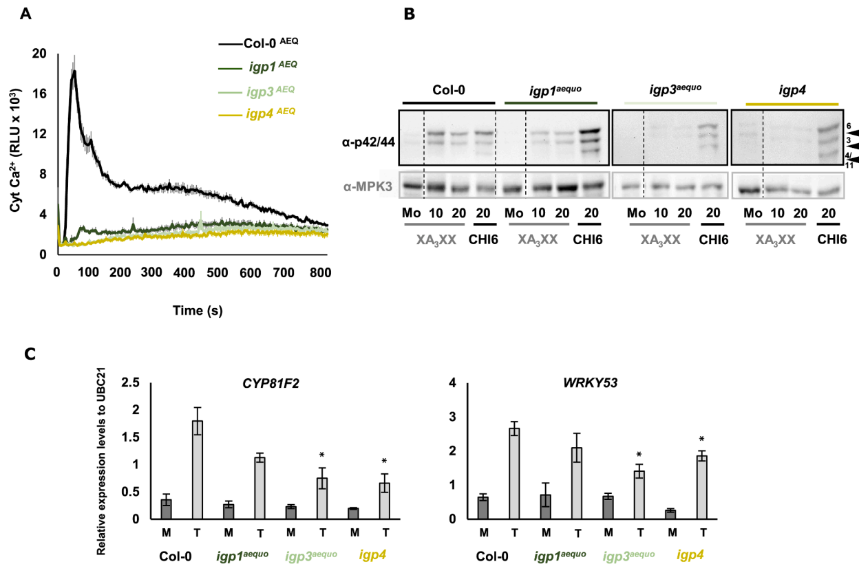
Fig. 4. igp1 , igp3 and igp4 mutants are impaired in \text{XA}_3\text{XX} perception. The activation of immunity hallmarks such as \text{cyt Ca}^{2+} influx (A) and phosphorylation of MPKs (B) is defective in igp mutants tested. Experiments were performed as described in Fig. 1. Data represent (A) the mean \pm error standard ( n = 8 ) of two independent experiments performed, (B) a representative WB out of three replicates (dotted lines indicate that bands were cut from the membrane to relocate them in proper order), and (C) the mean \pm error standard ( n = 3 ) of three independent experiments. Statistically significant differences between compound-treated (T) plants versus mock-treated (M, H 2 O) were calculated according to Student's t -test (* P < 0.05 , ** 0.01 < P < 0.001 , *** P < 0.001 ).
