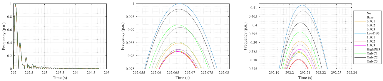
FIGURE 3. Absolute frequency deviation evolution under different control setups referred to the maximum value. Left plot shows the general evolution. Middle plot shows a detail of the first oscillation. Right plot shows a detail of the second oscillation.
