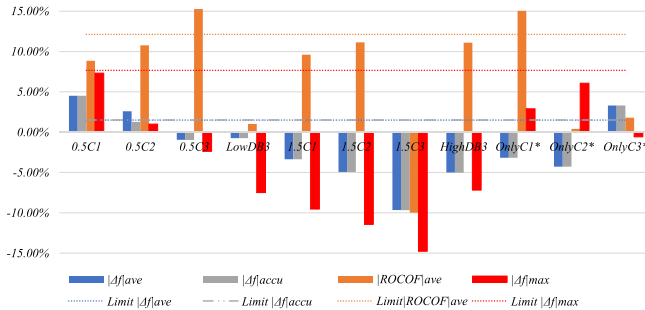
FIGURE 4. Experimental results: percentage metrics variation in control setups compared to base case (Section III) results. The dashed lines represent the limit of performance improvement.
