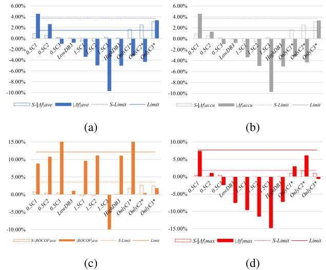
FIGURE 5. Comparison of experimental and simulation results. All the results are referred to the base setup described in Section III. The "S" denotes simulation results.
