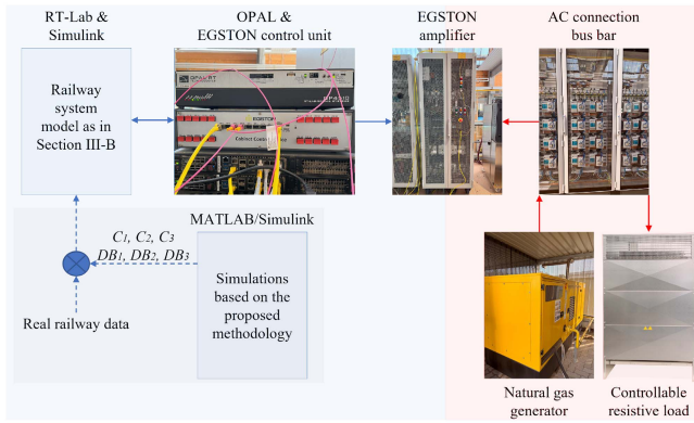
FIGURE 1. Interaction between simulation and experimental tests: power (red), data (blue), real-time flow (solid arrows), data transmittable online and offline (dashed arrows).
