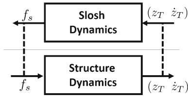
Fig. 4 Flowchart of the fluid–structure interaction problem
