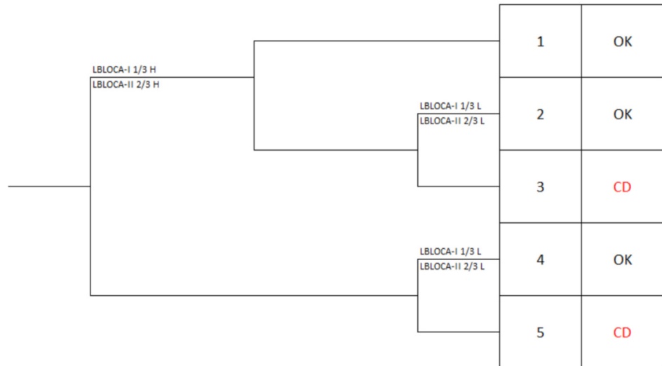
Fig. 17. Proposed LBLOCA-I and LBLOCA-II sequences Event Tree.
