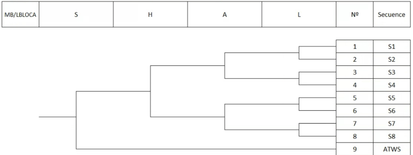
Fig. 10. MB/LBLOCA generic event tree.
