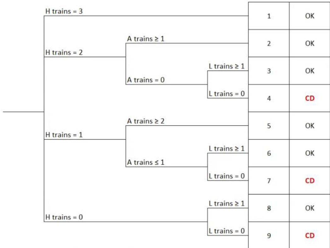
Fig. 19. LBLOCA-B expanded event tree.
