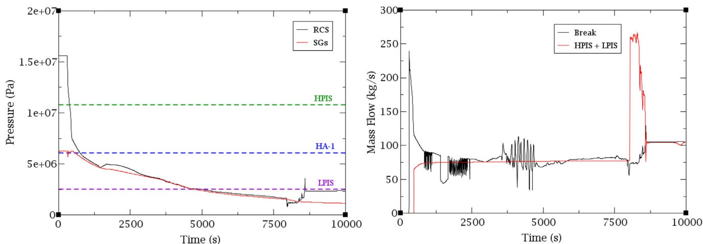
Fig. 6. RCS and SGs pressure (left) and RCS Inlet/Outlet mass flowrate (right); 2 inches MBLOCA reference sequence S-1/3H-2/4A-1/3L.
