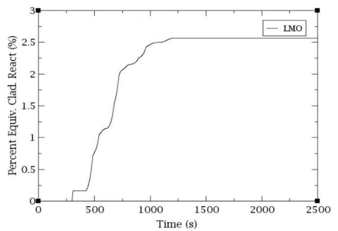
Fig. 8. RCS pressure (left) and Equivalent Cladding Reacted (right); DEGB LBLOCA reference sequence h-2/4A-1/3L.
