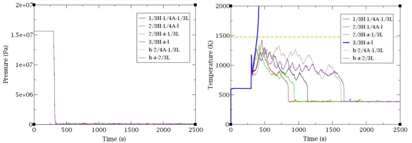
Fig. 14. RCS Pressure (left) and PCT (right); LBLOCA DEGB sequences.
