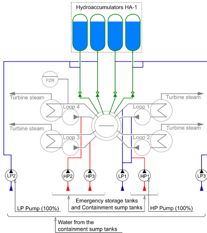
Fig. 1. ECCS configuration in VVER-1000/V320.
