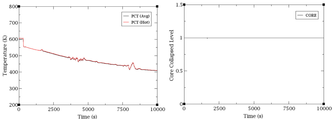
Fig. 7. PCT (left) and core collapsed liquid level (right); 2 inches MBLOCA reference sequence S-1/3H-2/4A-1/3L.
