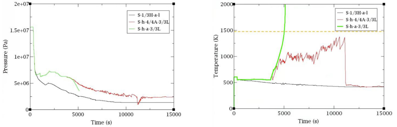
Fig. 12. RCS Pressure (left) and PCT (right); MBLOCA 2 inches sequences.
