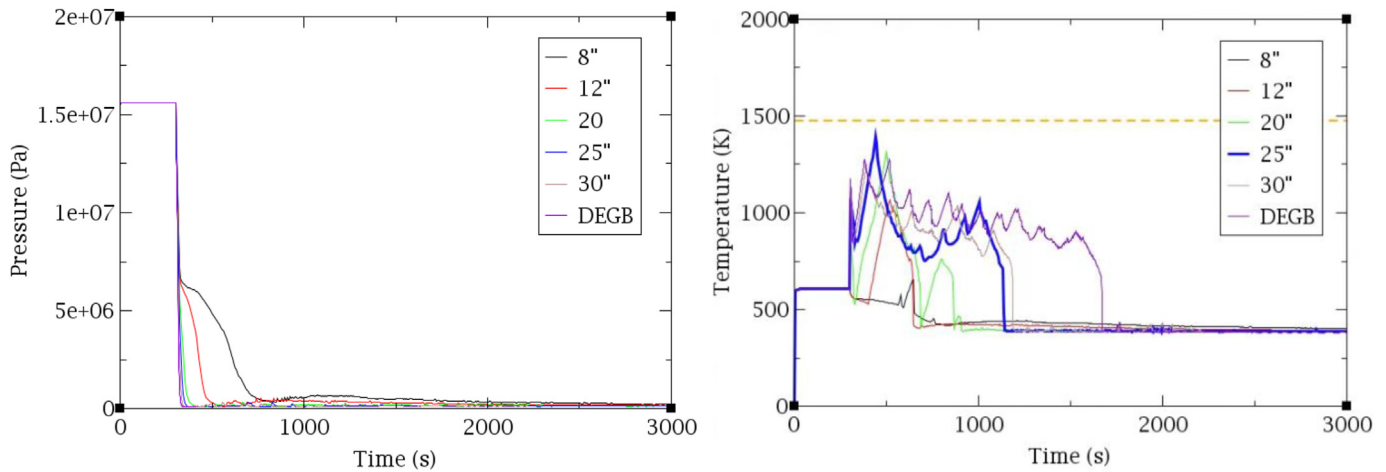
Fig. 13. RCS Pressure (left) and PCT (right); LBLOCA h-a-1/3L [8 inches–25 inches] and h-a-2/3L [30 inches-DEGB] sequence.
