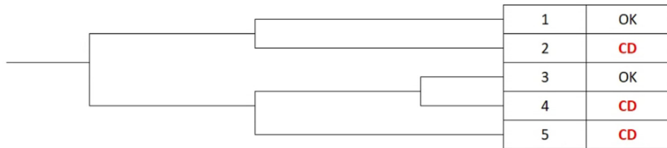
Fig. 3. Standard LBLOCA event tree of VVER1000/V320 [27].
