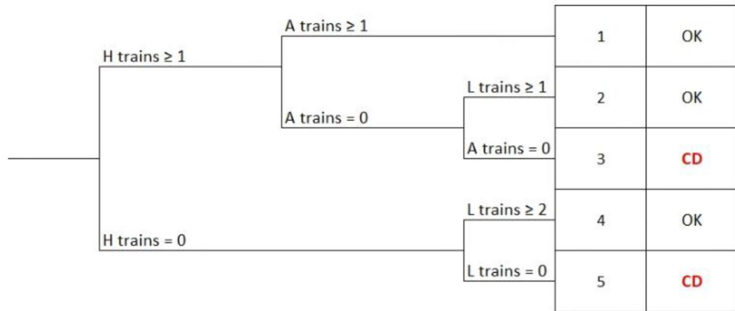
Fig. 20. LBLOCA-C expanded event tree.
