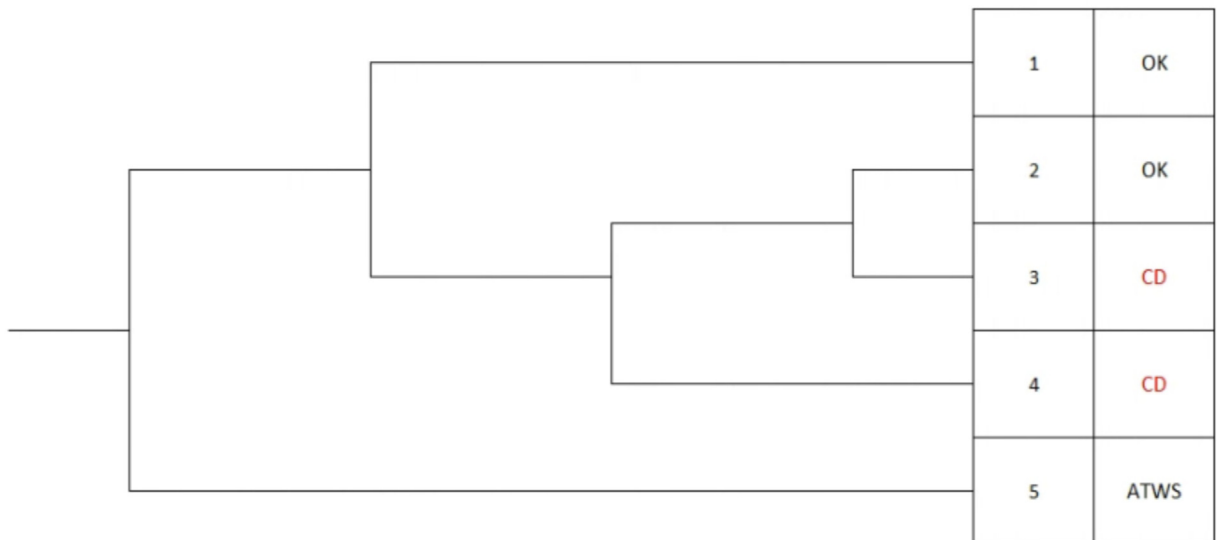
Fig. 15. Proposed MBLOCA-I sequences Event Tree.
