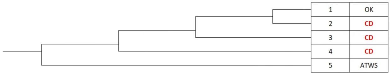
Fig. 2. Standard MBLOCA event tree of VVER-1000/V320 [27].
