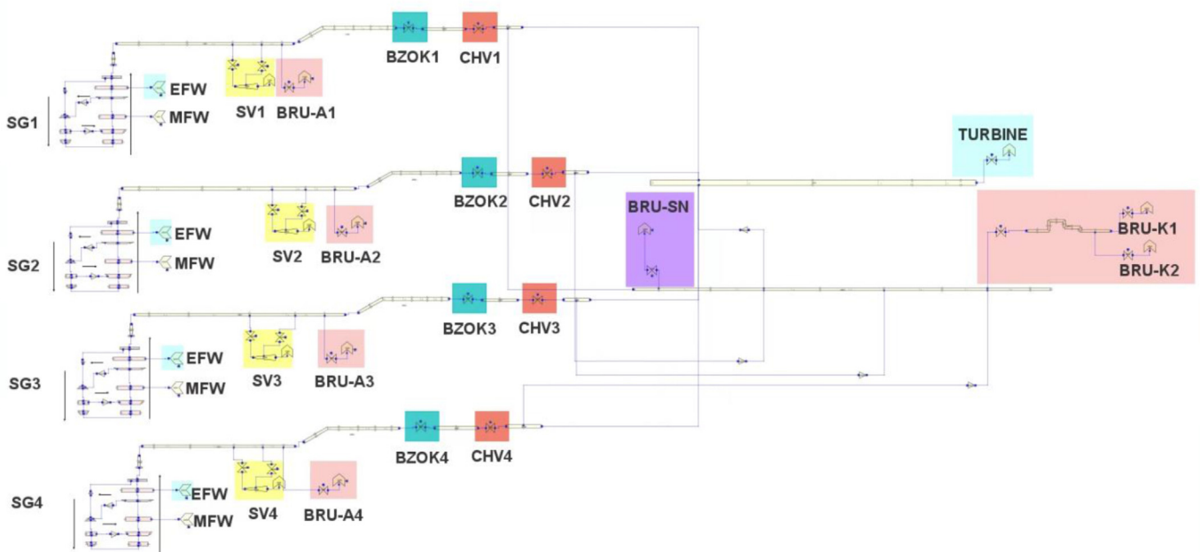
Fig. 5. Secondary side of VVER-1000/V320 TRACE TH model.
