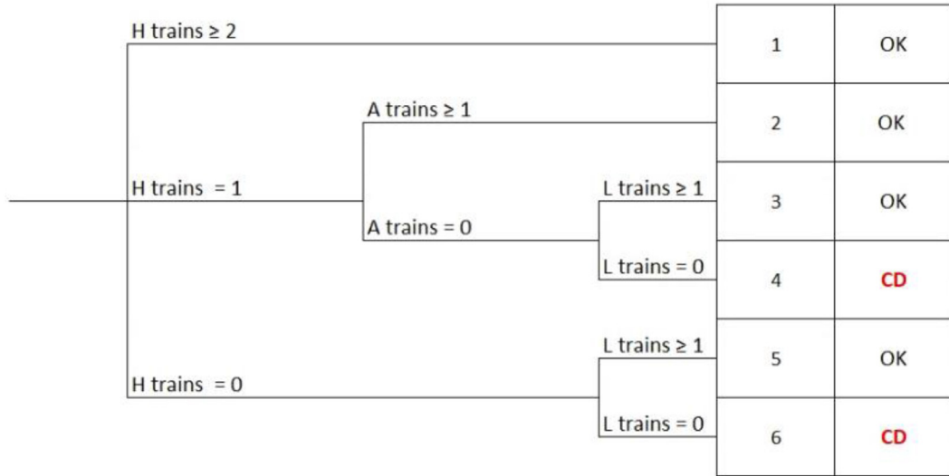
Fig. 18. LBLOCA-A expanded event tree.
