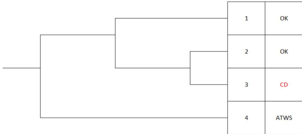
Fig. 16. Proposed MBLOCA-II sequences Event Tree.
