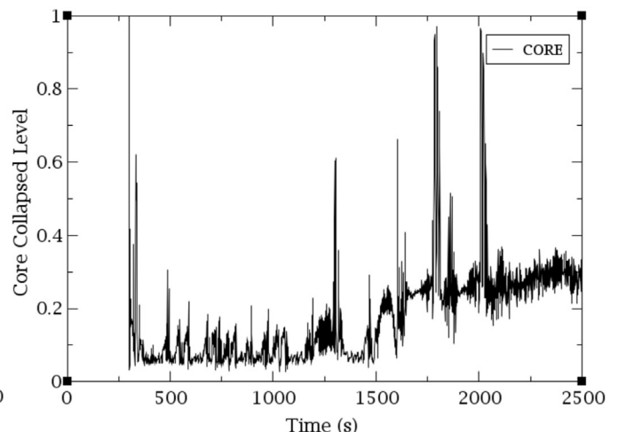
Fig. 9. PCT (left) and core collapsed liquid level (right); LBLOCA reference sequence h-2/4A-1/3L.
