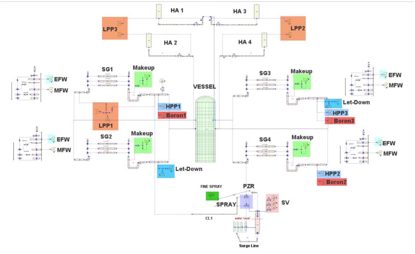
Fig. 4. Primary side of VVER-1000/V320 TRACE TH model.
