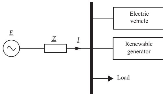
Figure 10.5 Simplified representation of a generic bus
