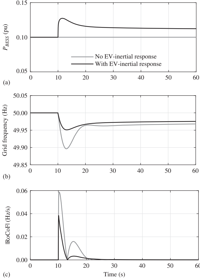
Figure 10.3 Time-domain simulation results: (a) Default EV-Battery charger operation mode (grey solid lines), (b) Frequency support provided by the EV-Battery charger (black solid lines)
