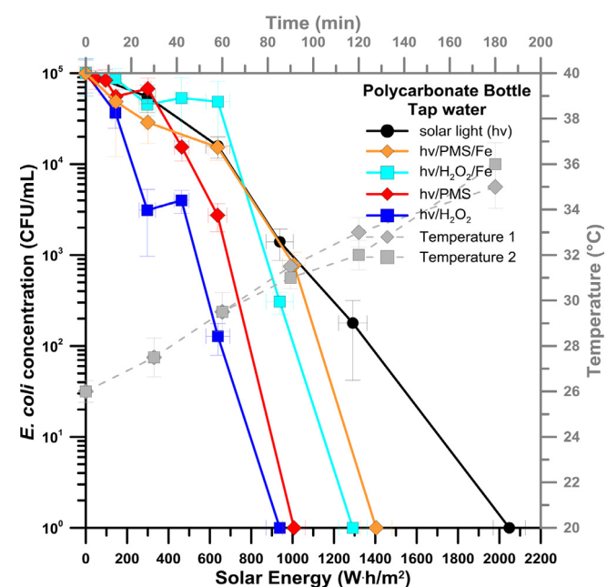
Fig. 2. Solar disinfection and enhancement experiments ( hv/H_2O_2 , hv/H_2O_2/Fe^{2+} , hv/PMS and hv/PMS/Fe^{2+} ) in the Polycarbonate bottle, with tap water. Initial concentrations of added reagents: [Fe^{2+}]_0 = 18 \mu M , [H_2O_2]_0 = 290 \mu M , [PMS]_0 = 36 \mu M . The vertical bars indicate the standard deviation from the mean bacterial concentration while the horizontal ones the SD of the received solar energy. Temperatures 1 and 2 (square and diamond traces) refer to the climatological conditions of the days when PMS or H_2O_2 based experiments took place, respectively (SODIS was always performed as control).
