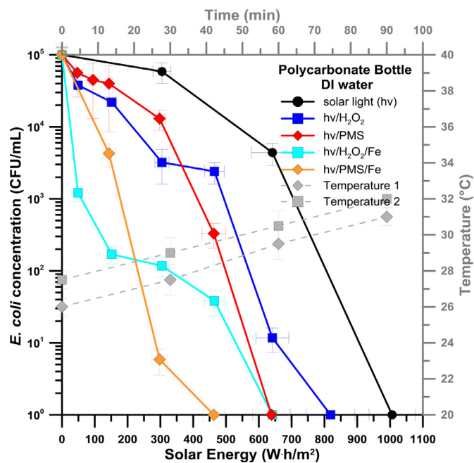
Fig. 1. Solar disinfection and enhancement experiments ( hv/H_2O_2 , hv/H_2O_2/Fe^{2+} , hv/PMS and hv/PMS/Fe^{2+} ) in the Polycarbonate bottle, with distilled water. Initial concentrations of added reagents: [Fe^{2+}]_0 = 18 \mu M , [H_2O_2]_0 = 290 \mu M , [PMS]_0 = 36 \mu M . The vertical bars indicate the standard deviation from the mean bacterial concentration while the horizontal ones the SD of the received solar energy. Temperatures 1 and 2 (square and diamond traces) refer to the climatological conditions of the days when PMS or H_2O_2 based experiments took place, respectively (SODIS was always performed as control).
