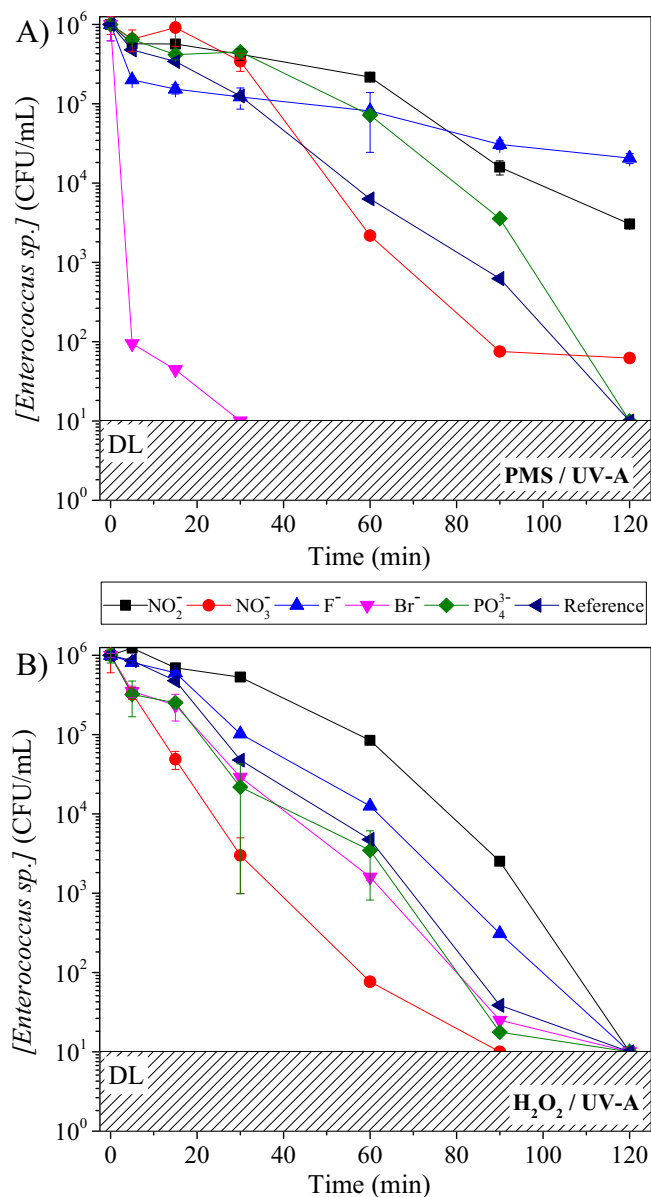
Fig. 8. Influence of the presence of inorganic anions on PMS (A) and \text{H}_2\text{O}_2 (B) photoactivation for Enterococcus sp. inactivation. Experimental conditions: [PMS] = 0.05 mM; [ \text{H}_2\text{O}_2 ] = 1.5 mM; pH = natural; Matrix = DW; Reactor = tubular reactor; Irradiation = UV-A.
