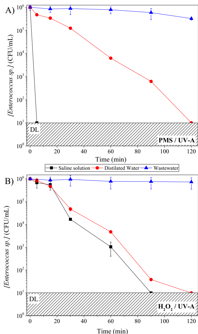
Fig. 4. Influence of the matrix on the photoactivation of PMS (A) and \text{H}_2\text{O}_2 (B) for the inactivation of Enterococcus sp. Experimental conditions: [\text{PMS}] = 0.05 \text{ mM} ; [\text{H}_2\text{O}_2] = 1.5 \text{ mM} ; pH = natural; Reactor = tubular reactor; Irradiation = UV-A.
