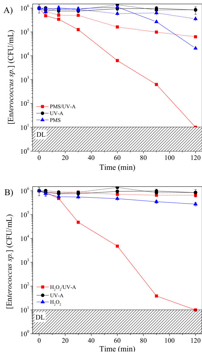
Fig. 2. Influence of the reactor on A) PMS and B) \text{H}_2\text{O}_2 for the inactivation of Enterococcus sp. (solid lines: tubular reactor; dashed lines: batch reactor). Experimental conditions: [PMS] = 0.05 mM; [ \text{H}_2\text{O}_2 ] = 1.5 mM; pH = natural; Matrix = distilled water; Irradiation = UV-A.
