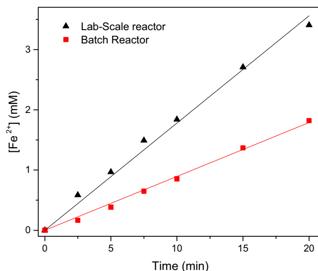
Fig. 3. Variation of \text{Fe}^{2+} concentration during ferrioxalate actinometry experiments for a batch and a tubular reactor.
