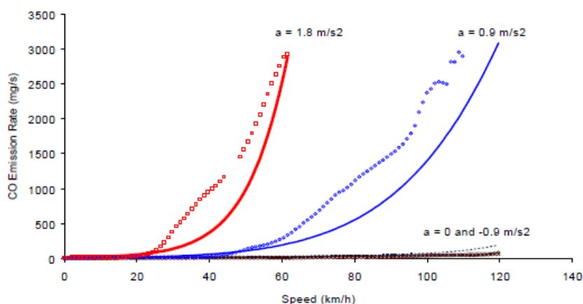
Figure 2. Regression fit for CO emissions as a function of speed and acceleration rates. Source [34]
