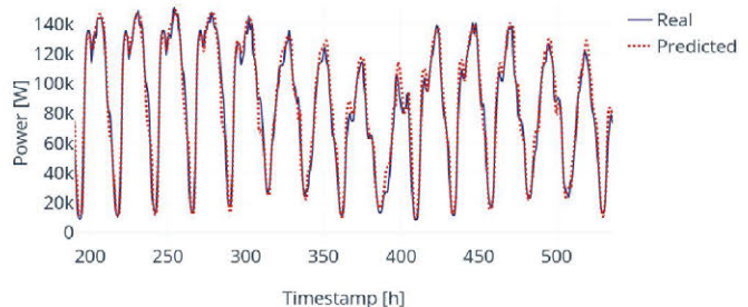
Fig. 6. Power prediction for Stacked Off strategy
