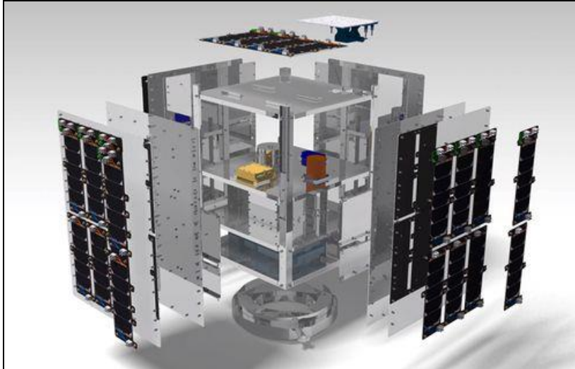
Figure 2. Exploited 3D model of the UPMSat-2
