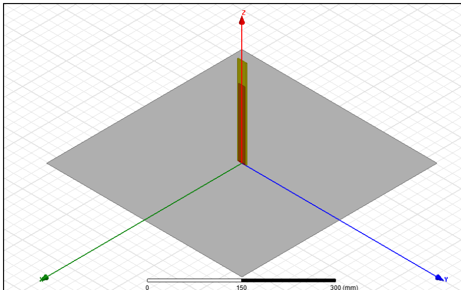
Figure 3. Simulation model of the UPMSat-2 monopole using ANSYS HFSS® software. It includes the monopole and the support satellite tray
