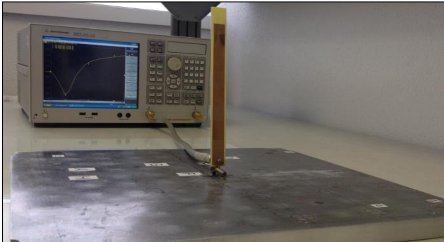
Figure 4. Test model of the UPMSat-2 monopole used to validate the results obtained with the simulation model
