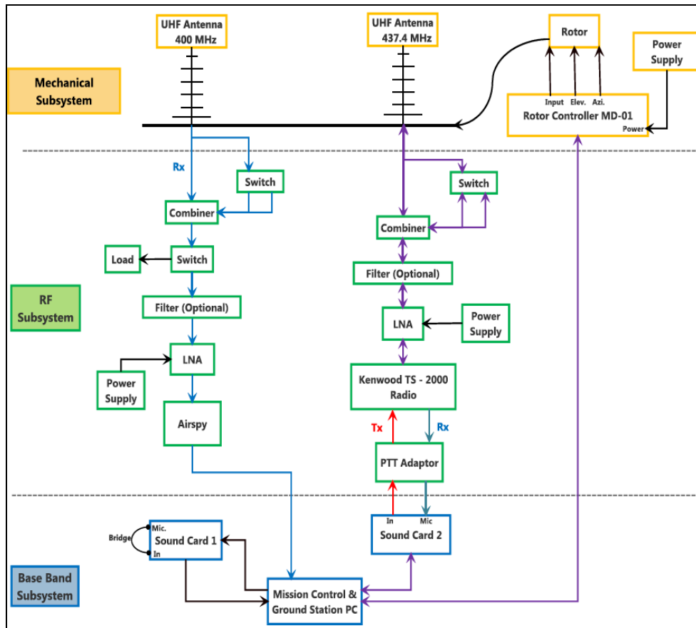
Figure 9. UPM Ground Station Architecture (Option 1)
