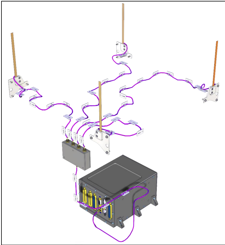
Figure 7. Isometric view of the complete communication subsystem equipment and harness
